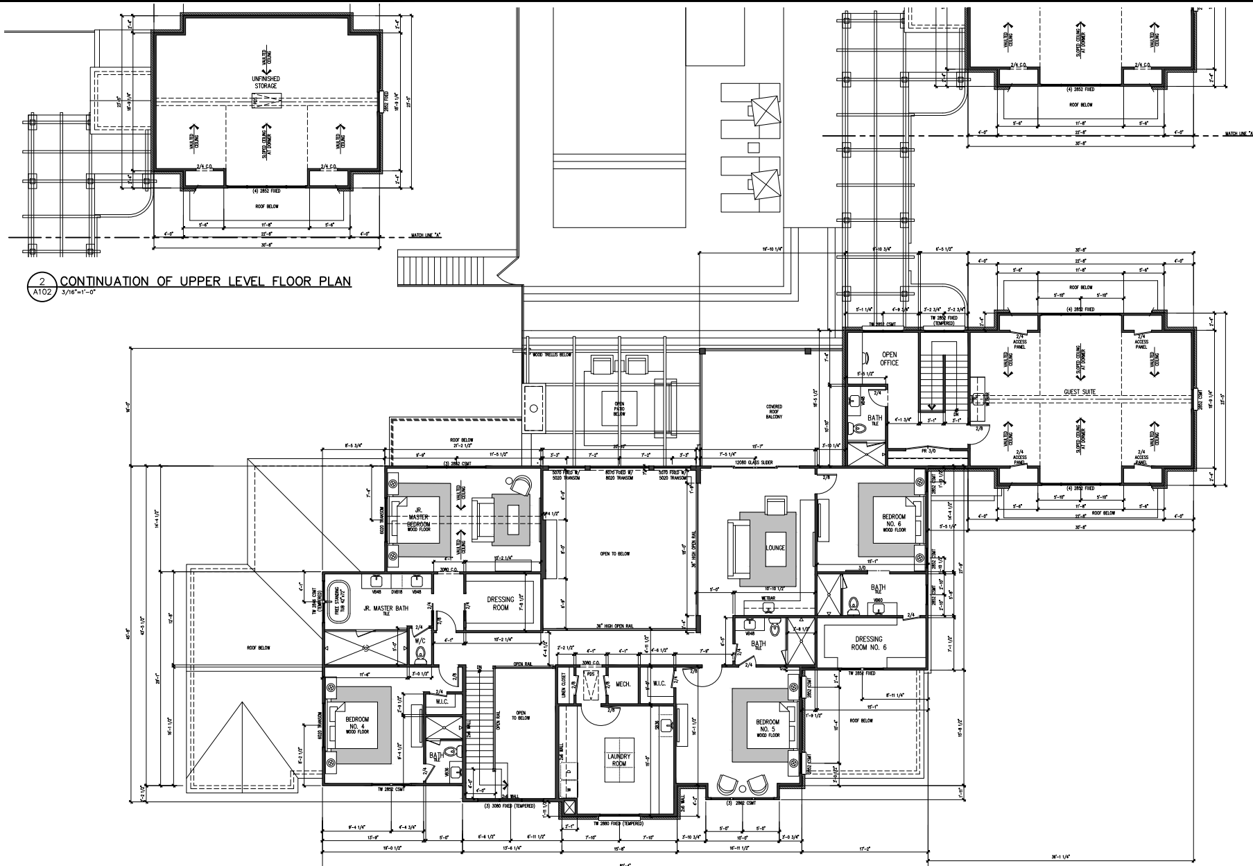
1 UPPER LEVEL FLOOR PLAN 3/16"=1'-0"
