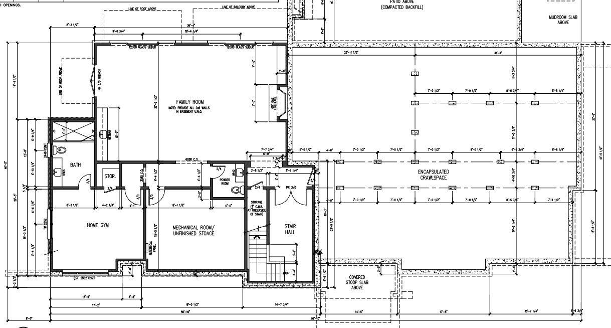
1 BASEMENT LEVEL FLOOR PLAN A100 3/16"=1'-0"
