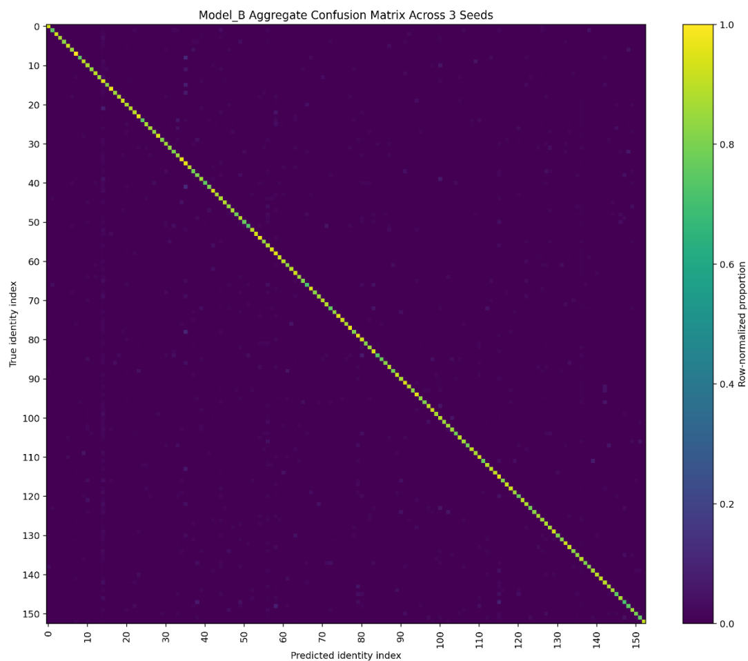
Fig. A5. Aggregate row-normalized confusion matrix for the pose-diverse Model B across the three random-seed runs.
