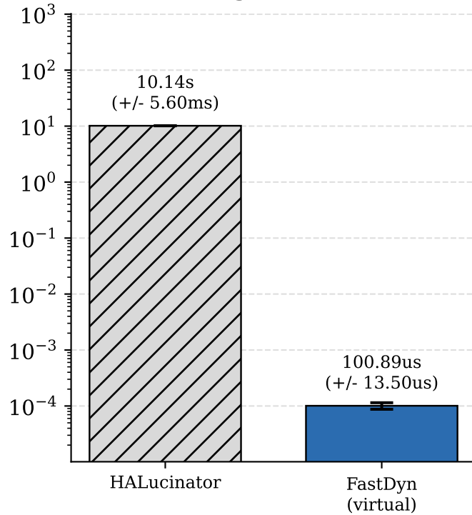
Slicing (Counter)
