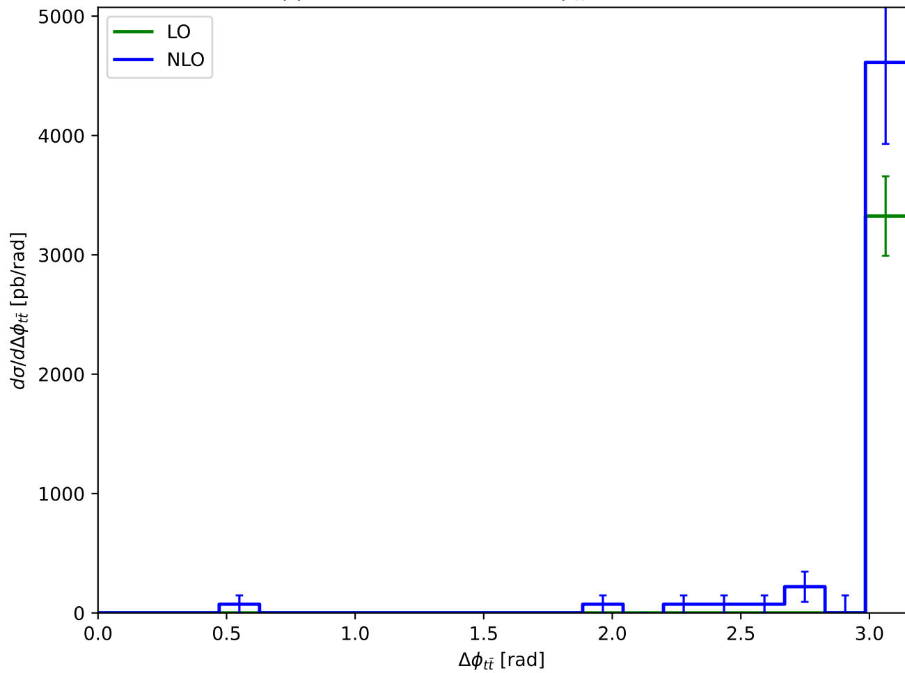
pp \rightarrow t\bar{t} at \sqrt{s} = 13 TeV: \Delta\phi_{t\bar{t}} distribution
