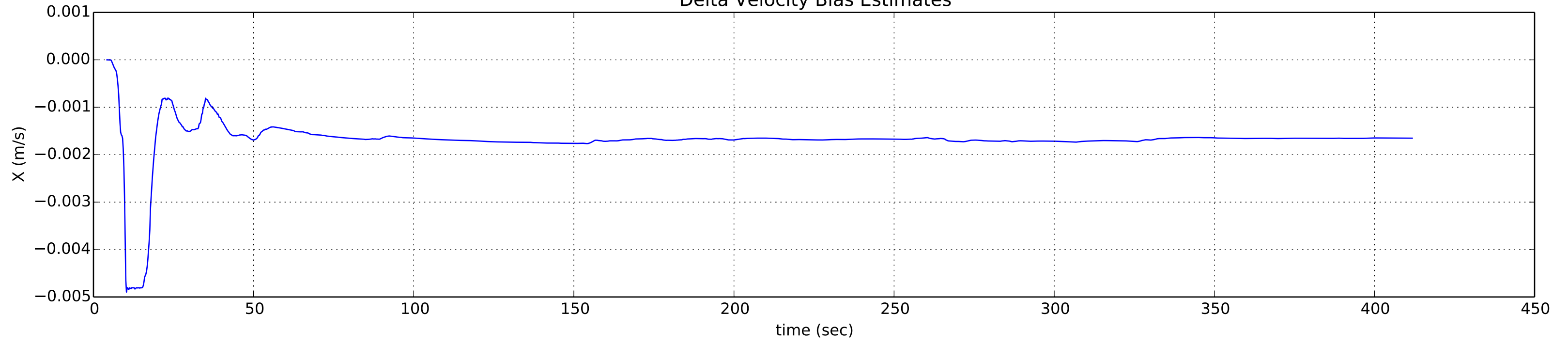
Delta Velocity Bias Estimates
