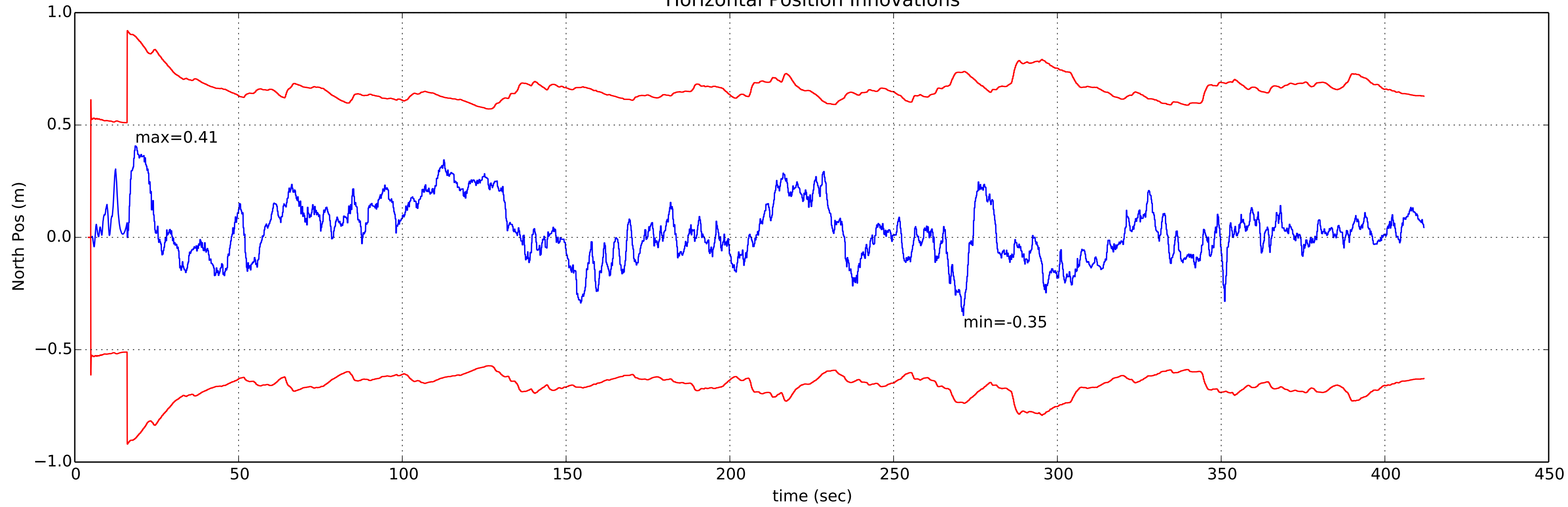
Horizontal Position Innovations
