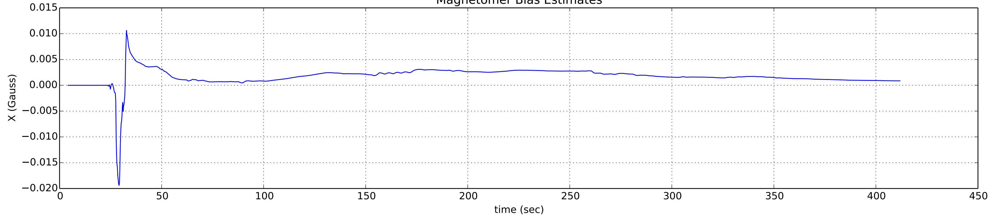
Magnetomer Bias Estimates
