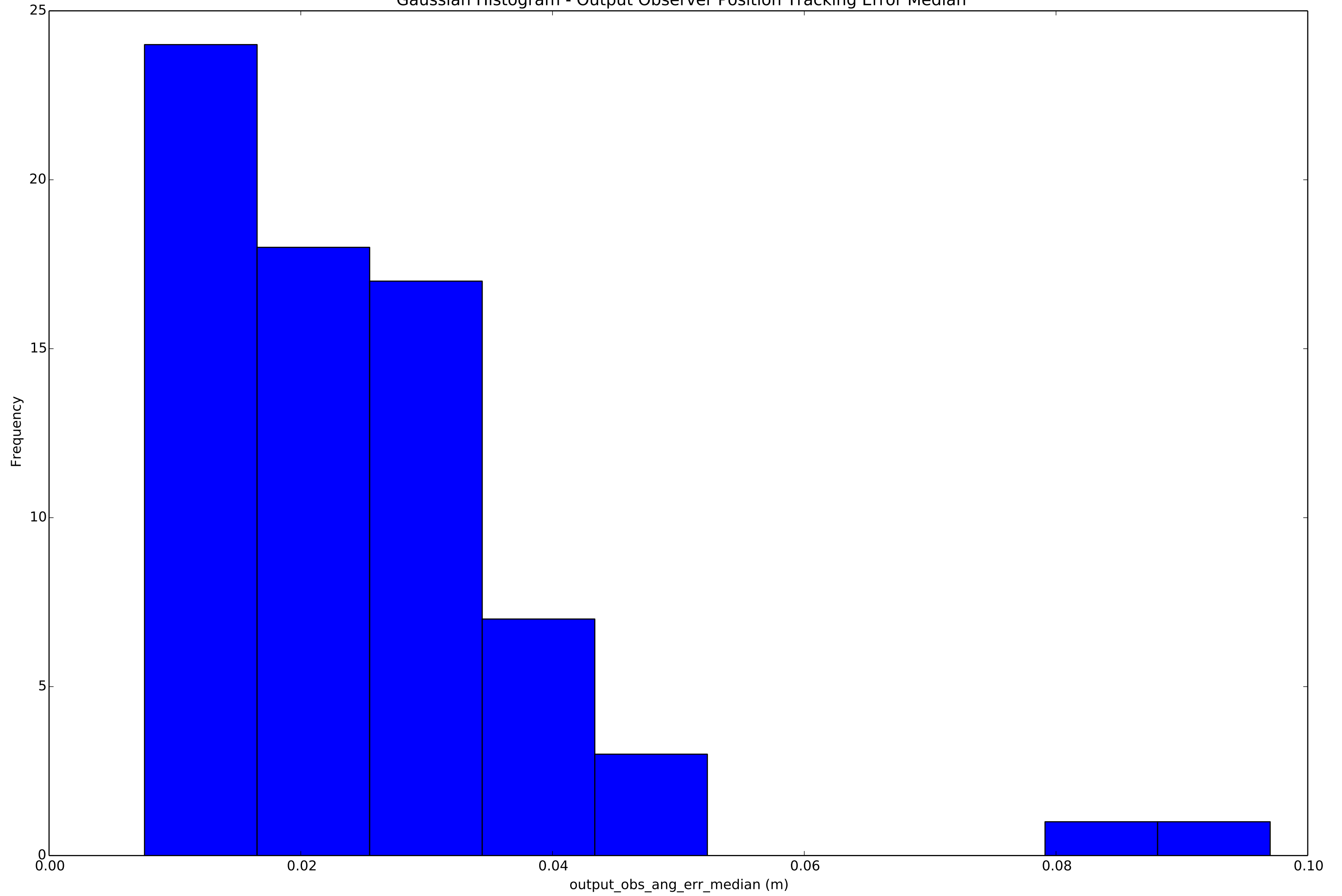
Gaussian Histogram - Output Observer Position Tracking Error Median
