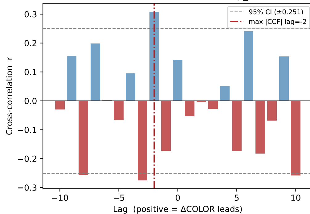
(c) CCF diffs: \Delta COLOR vs. \Delta ucdp_wars
