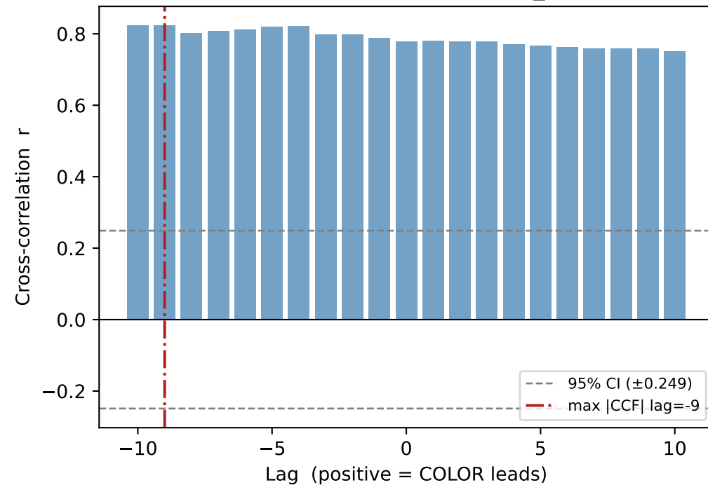
(b) CCF levels: COLOR vs. ucdp_smooth
