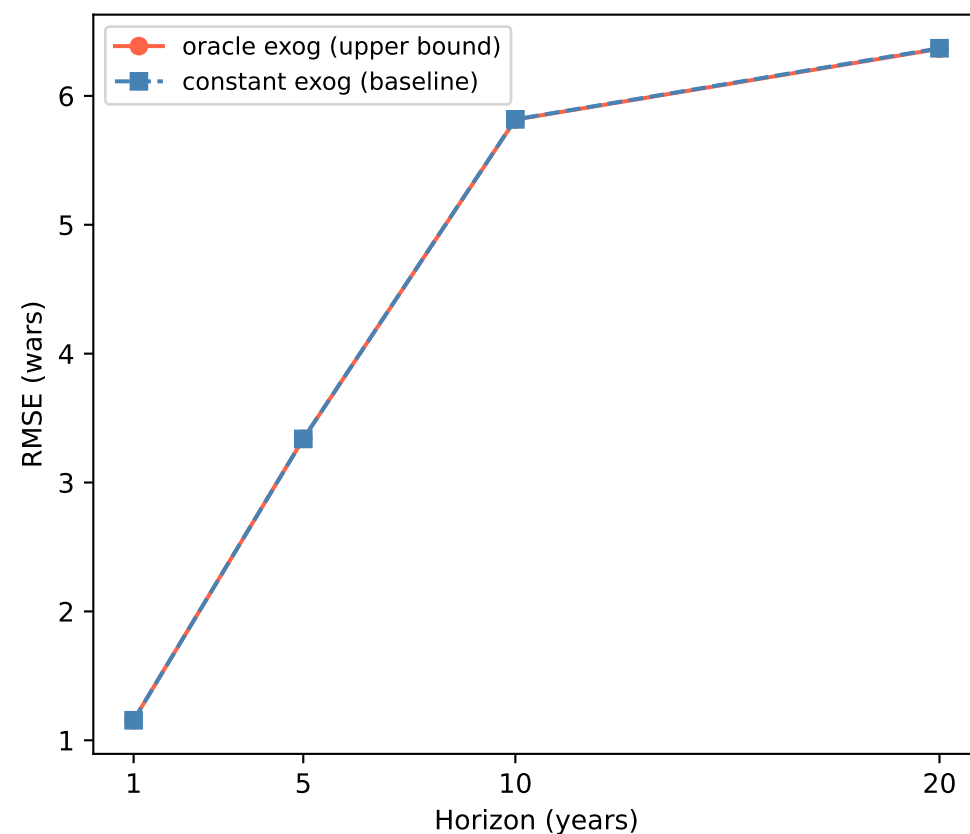
RMSE vs. forecast horizon
