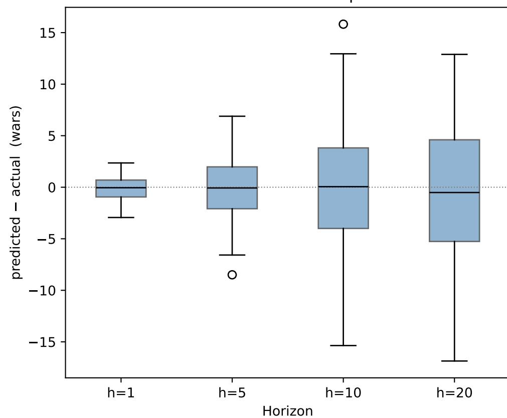
Forecast error distribution per horizon
