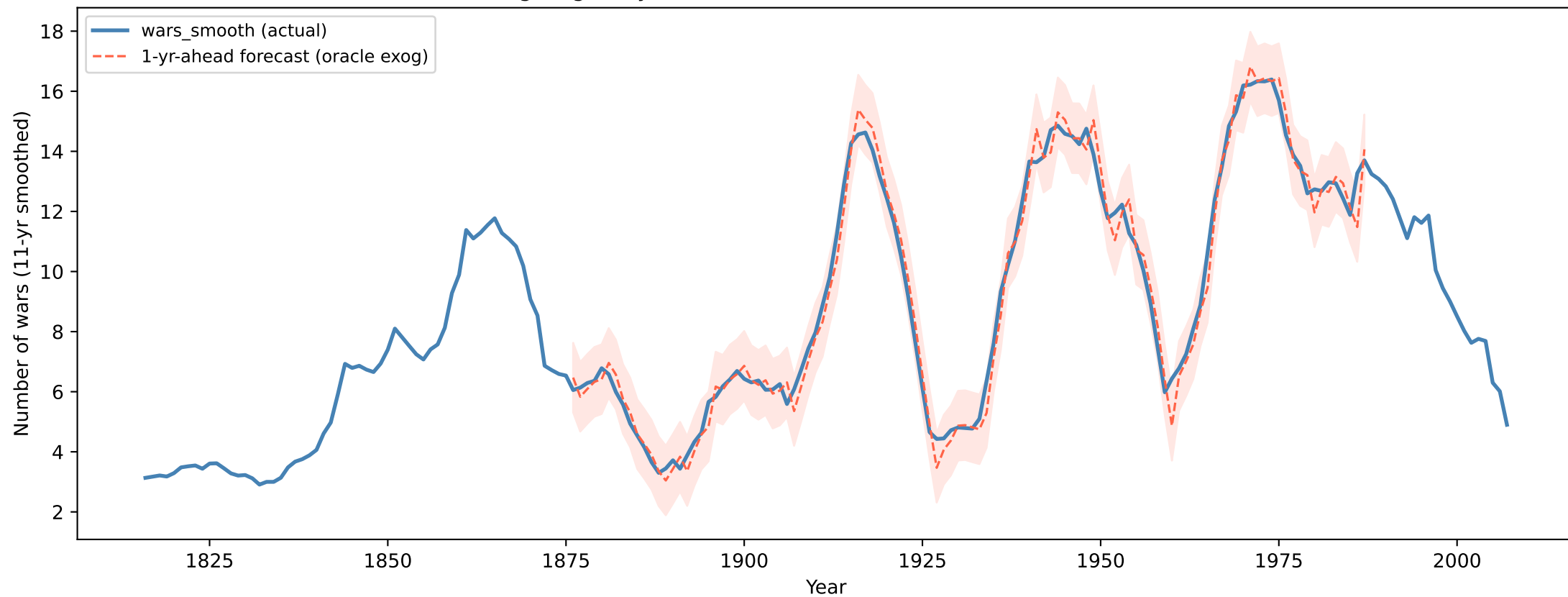
Rolling-origin 1-year-ahead forecasts vs. actual [ARIMAX(1,1,1)]
