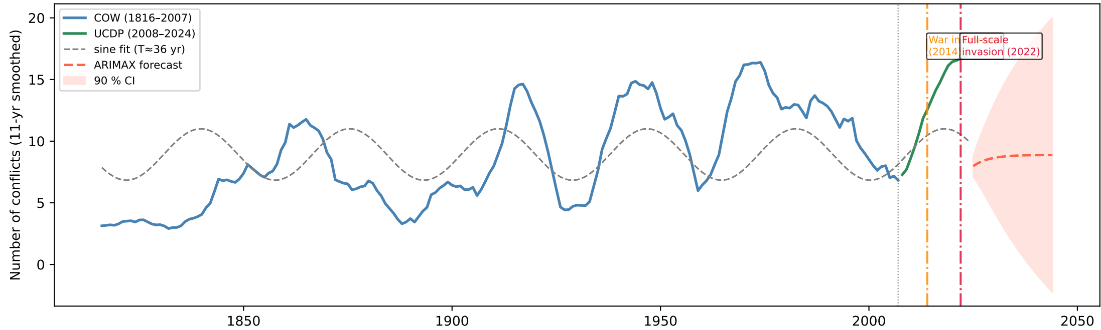
CPS - extended series COW (1816-2007) + UCDP v25.1 (2008-2024) ARIMAX(1,1,1) + COLOR exog | sine period \approx 36 yr
