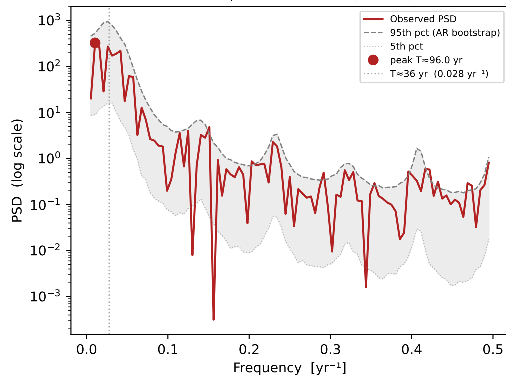
(b) wars_smooth — AR(13) bootstrap Observed peak within 95% CI [B=2000]
