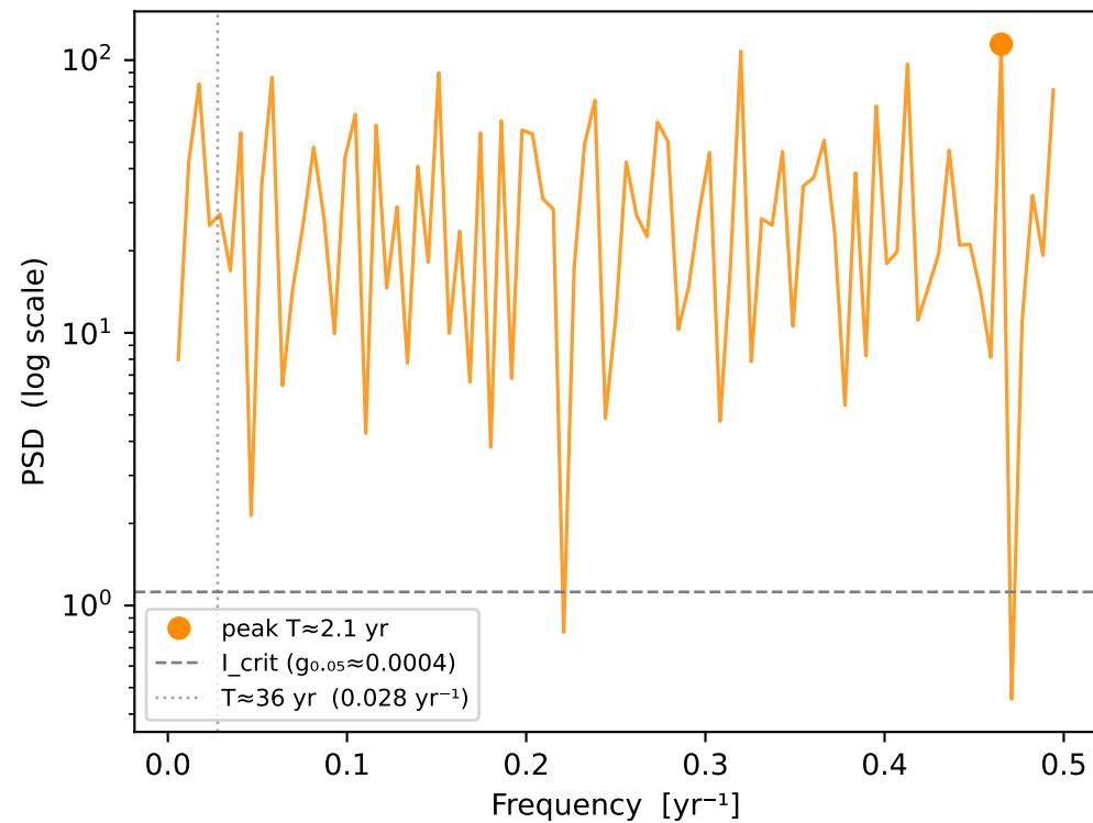
(c) wars (raw) AR(20) residuals — Fisher g-test g=0.0420 , p = 0.9474 n.s. [after prewhitening]
