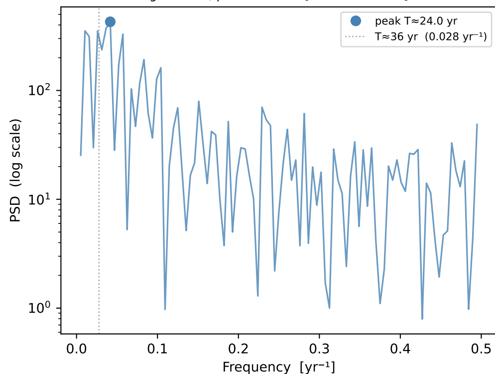
(a) wars (raw) — Fisher g-test g=0.0854 , p = 0.0214 * [white-noise null]
