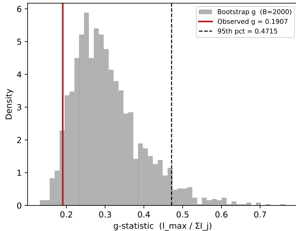
(d) wars_smooth: bootstrap p-value for g-stat p_{boot} = 0.9505 \rightarrow not significant [AR(13) null]
