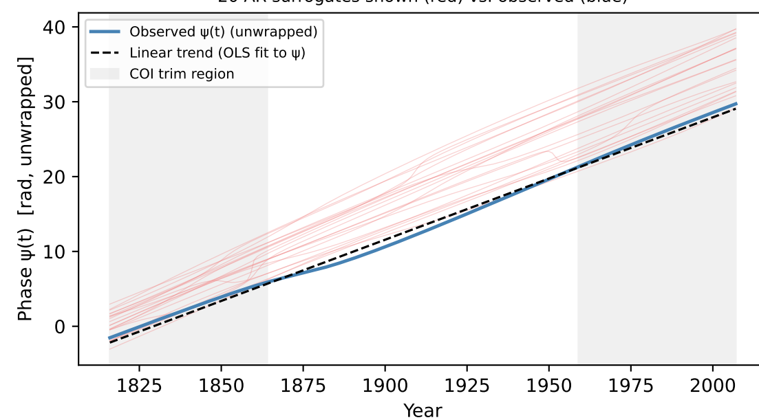
(C) Instantaneous phase at T\approx 35.1 yr 20 AR surrogates shown (red) vs. observed (blue)
