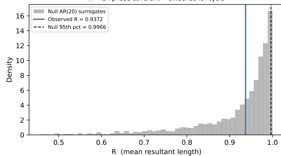
(E) Phase coherence R — 192 obs, AR(20) p_R = P(\text{null} \geq \text{obs}) = 0.6155 [n.s.] R \rightarrow 1 : phase coherent \rightarrow evidence for cycle
