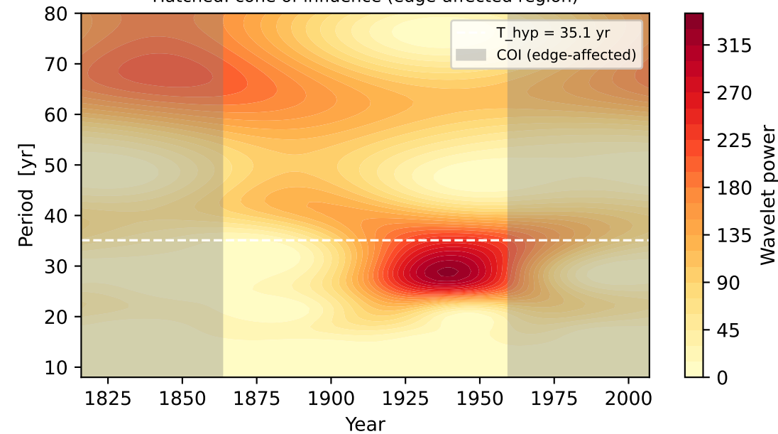
(B) Wavelet power scalogram (Morlet, \omega_0=6 ) Hatched: cone of influence (edge-affected region)
