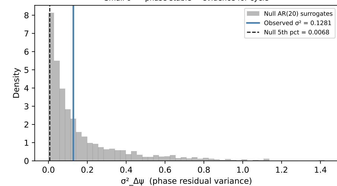
(D) Phase variance — 192 obs, AR(20) p_{\sigma^2} = P(\text{null} \leq \text{obs}) = 0.6145 [n.s.] Small \sigma^2 \rightarrow phase stable \rightarrow evidence for cycle
