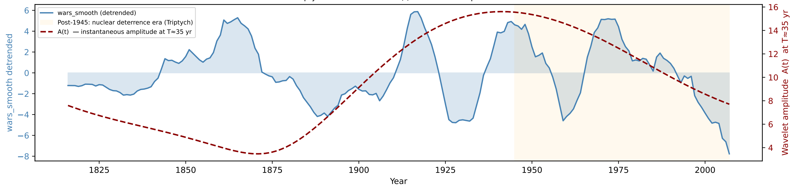
(A) Instantaneous amplitude A(t) at T\approx 35.1 yr [scale s\approx 33.5 , Morlet \omega_0=6 ] If Triptych model is correct: A(t) should decline post-1945
