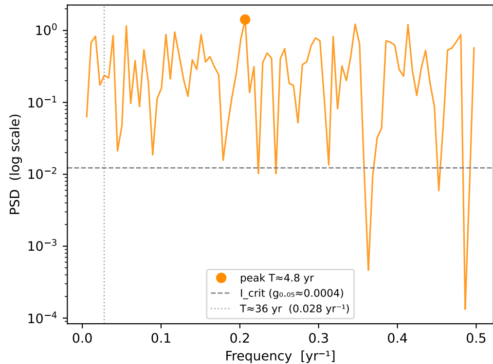
(c) wars_smooth AR(13) residuals — Fisher g-test g=0.0435 , p = 0.8851 n.s. [after prewhitening]
