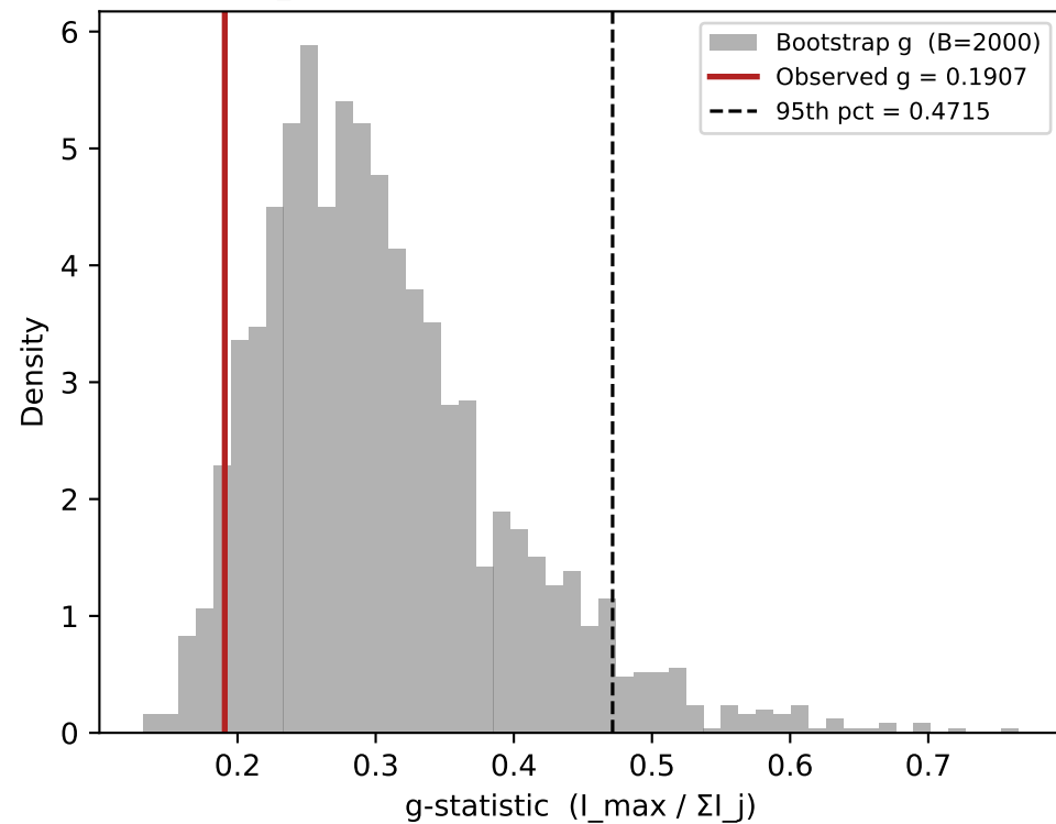
(d) wars_smooth: bootstrap p-value for g-stat p_{\text{boot}} = 0.9505 \rightarrow not significant [AR(13) null]
