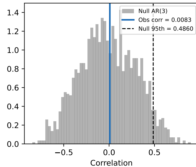
(C) Out-of-sample corr (epoch 2) p = 0.4690 [n.s.]
