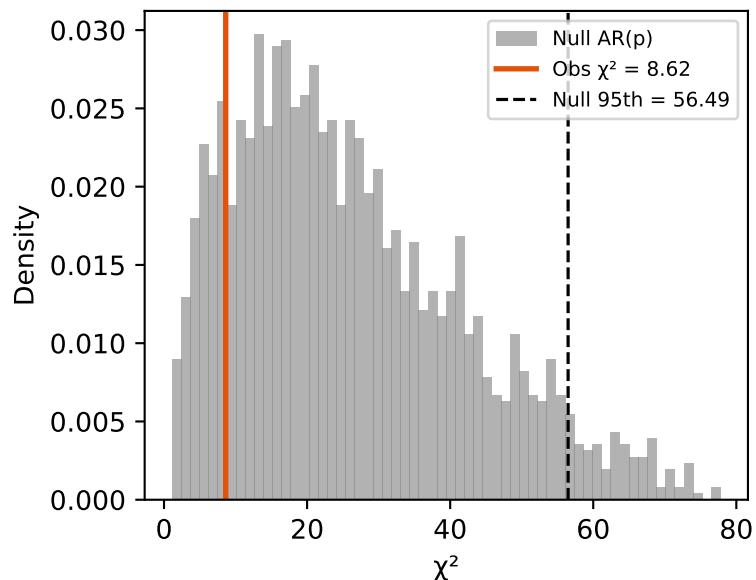
(A) Epoch-fold: 1816–1913 AR(3), p = 0.8655 [n.s.]
