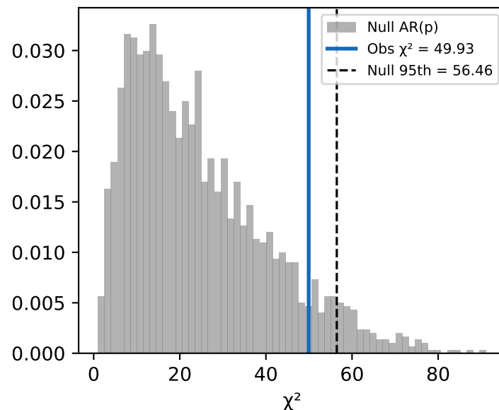
(B) Epoch-fold: 1914–2024 AR(3), p = 0.0865 [n.s.]
