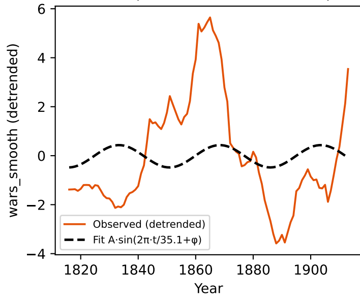
(D) Sinusoid fit — epoch 1 (1816–1913) Phase and amplitude locked here, tested in epoch 2
