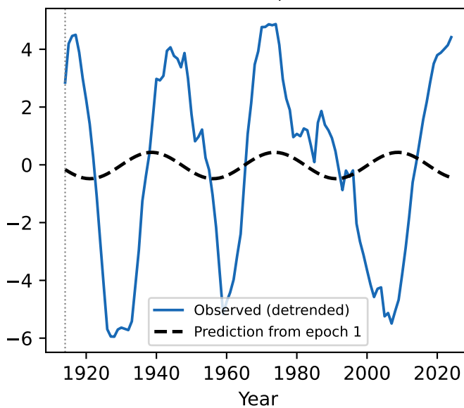
(E) Out-of-sample prediction — epoch 2 (1914–2024) corr = 0.0083, p = 0.4690
