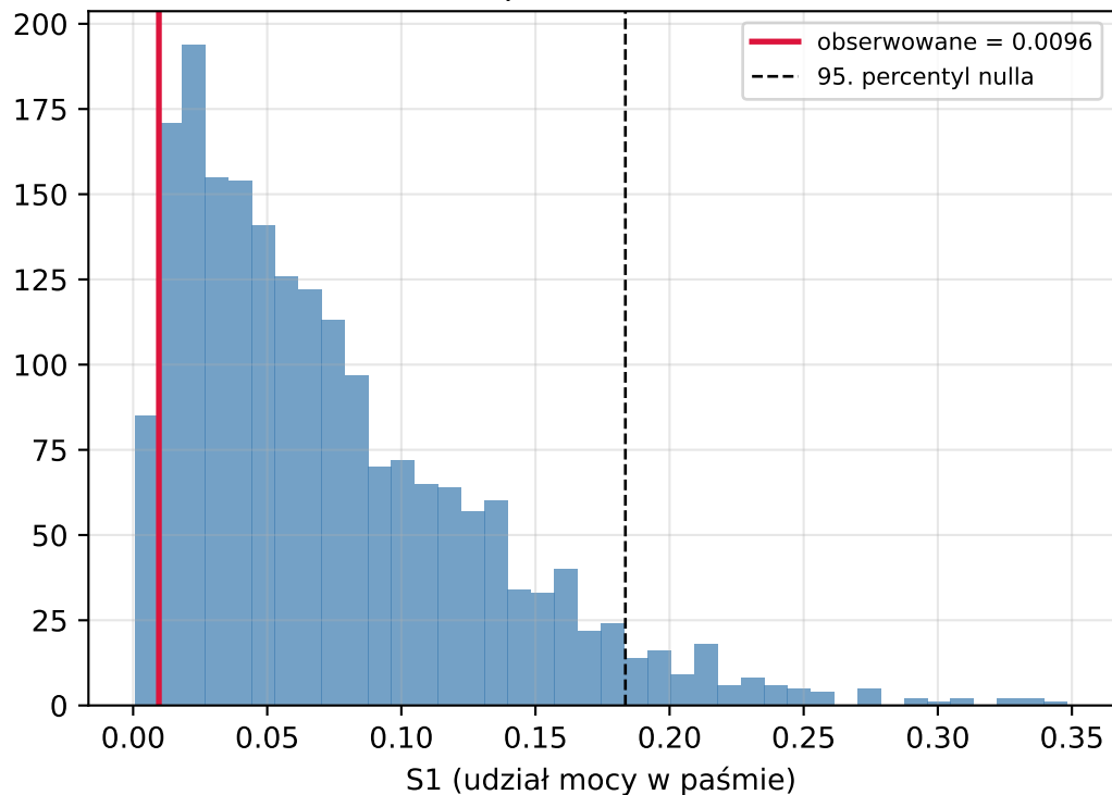
Panel 3a. P1 — null: AR(3) p = 0.9555
