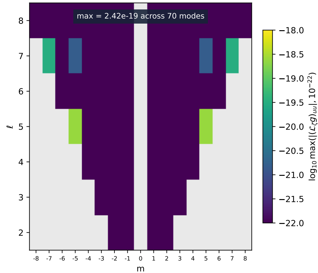
Helical: \omega = m\Omega
