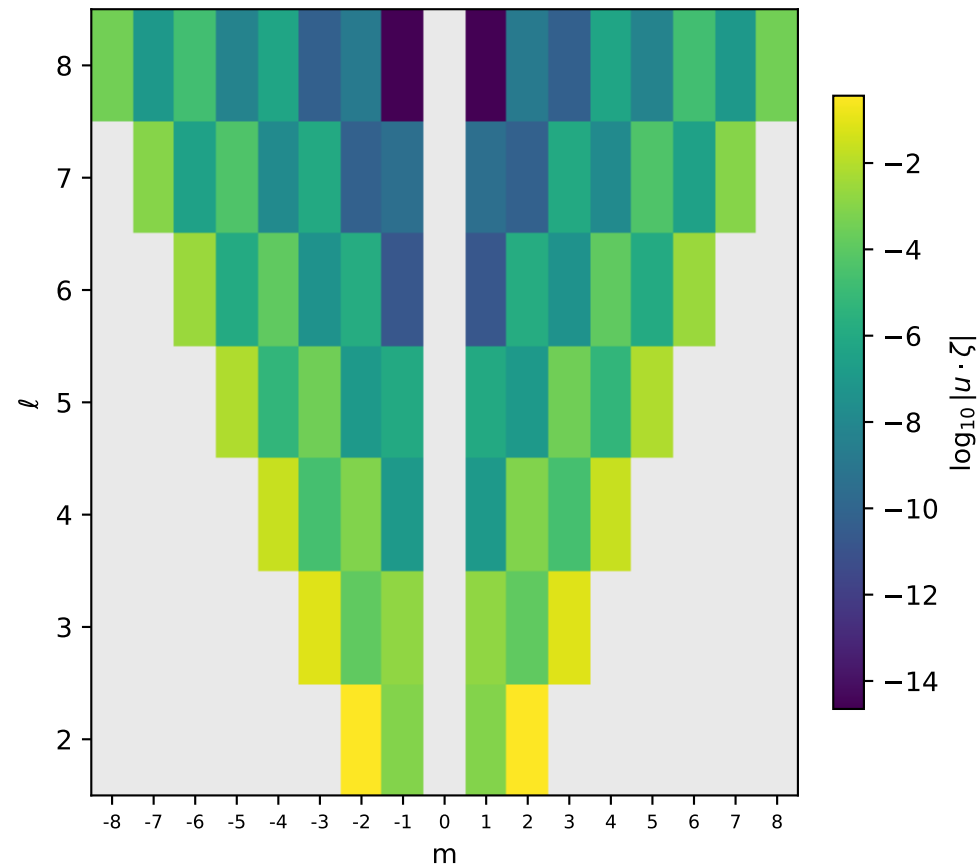
Gauge-vector contraction |u \cdot \zeta|
