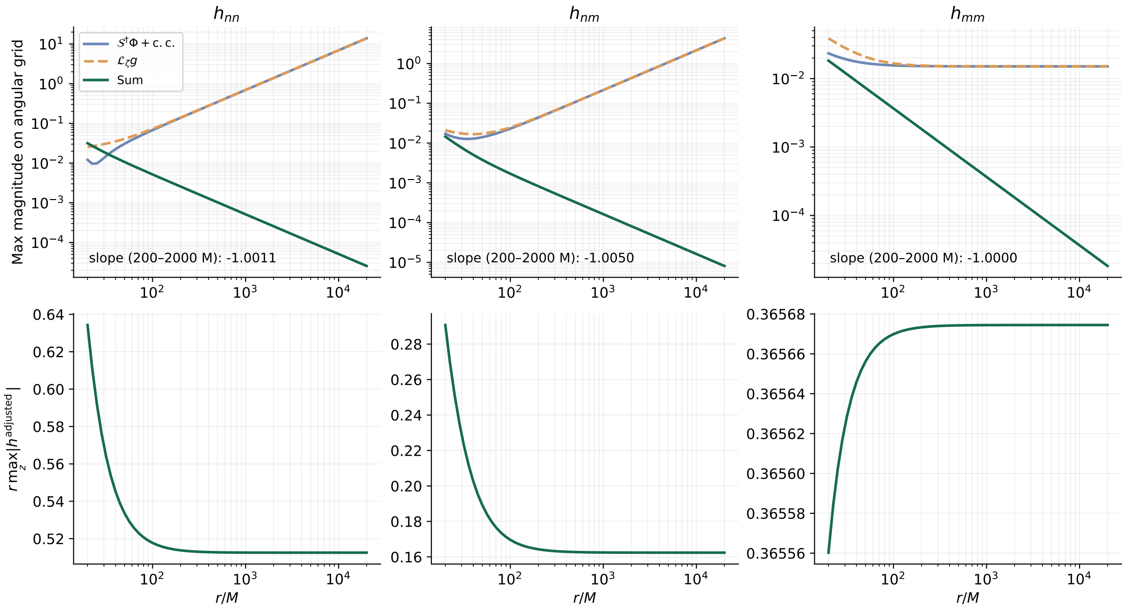
Circular Kerr orbit: a/M = 0.5 , r_0/M = 10 , m = 2 SN source \ell = 2 \dots 8 ; angular m-mode solve, N_z = 13 ; M = \mu = 1
