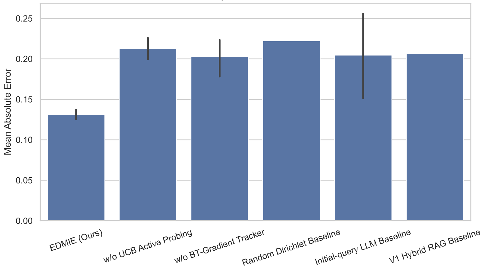
Preference Alignment Error Across Baselines
