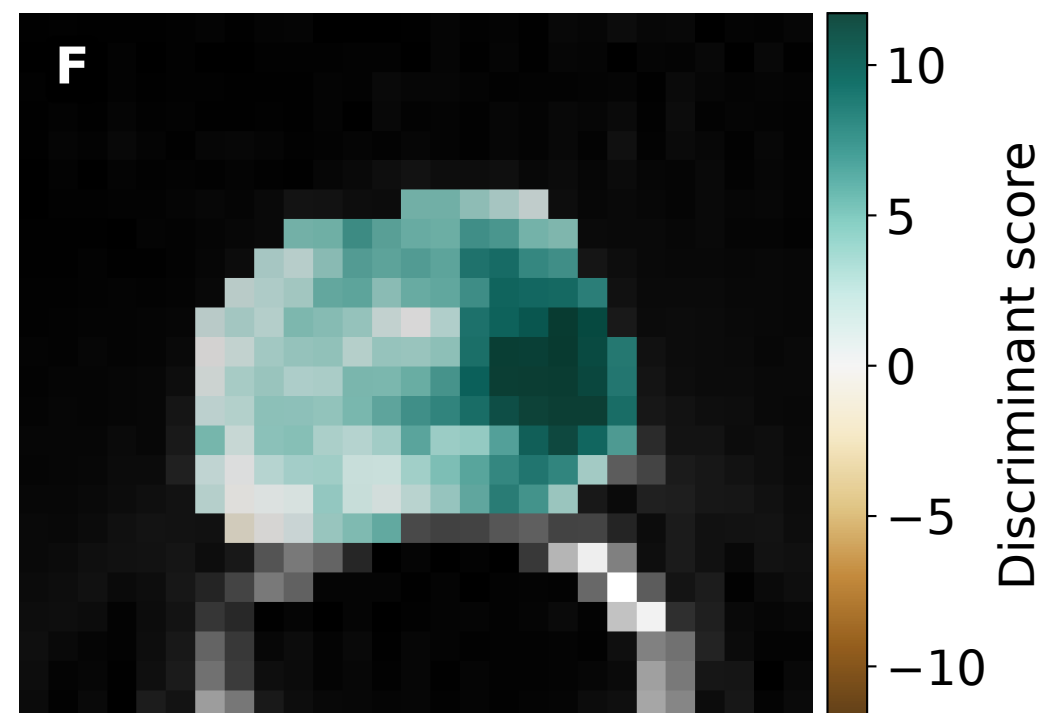
8-Bin Score
