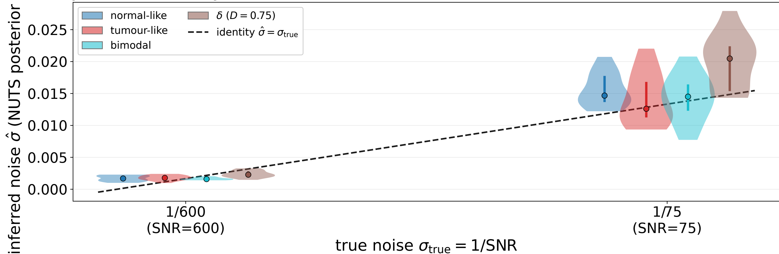
joint noise recovery — \hat{\sigma} vs \sigma_{\text{true}} (violins over noise realizations)
