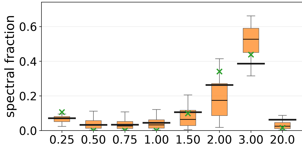
normal-like, SNR=75 — \hat{R}=1.00
