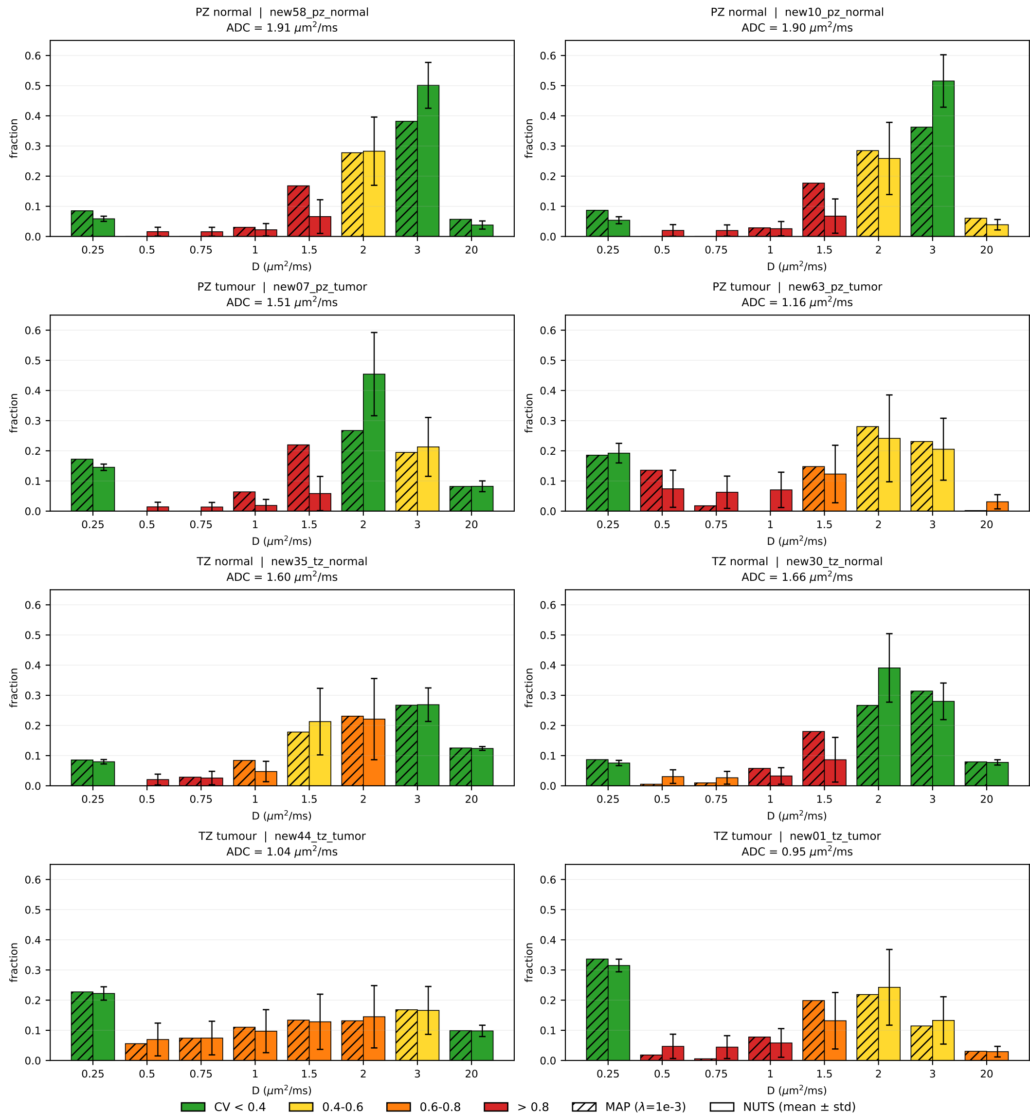
Tuned MAP ( \lambda=1e-3 , hatched) vs NUTS (solid + posterior \pm 1 sd) — 8 representative ROIs, bars coloured by NUTS posterior CV
