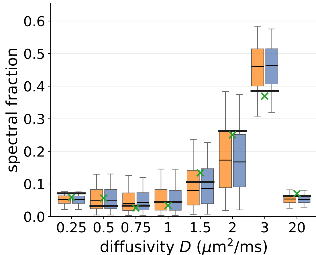
(a) normal-like spectrum
