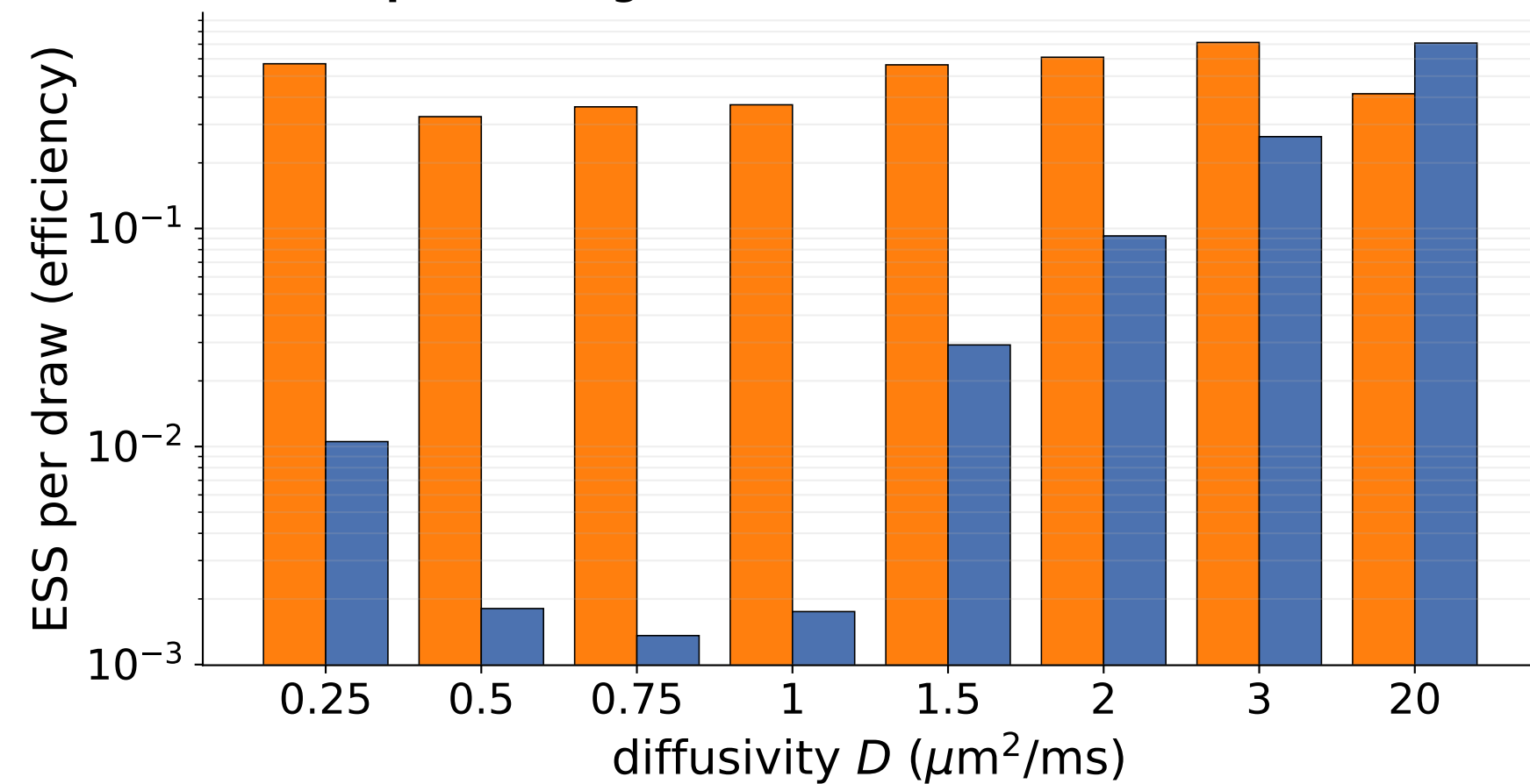
(e) sampler mixing ( \delta stress)
