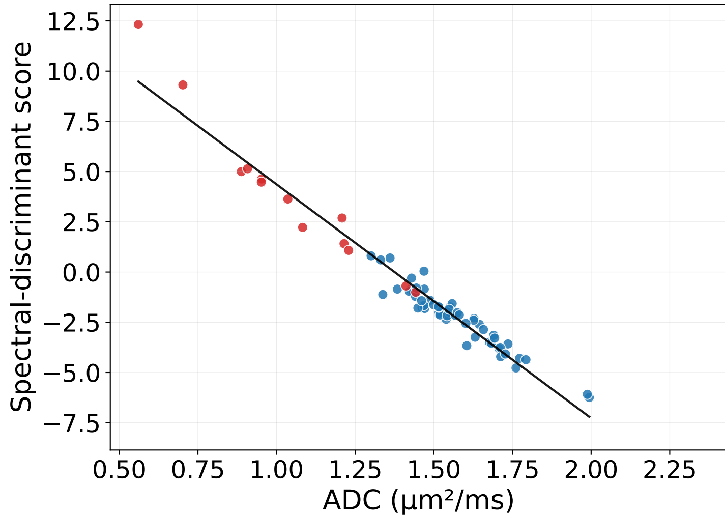
TZ — NUTS (posterior mean) r = -0.979 [-0.988, -0.971] , n = 68
