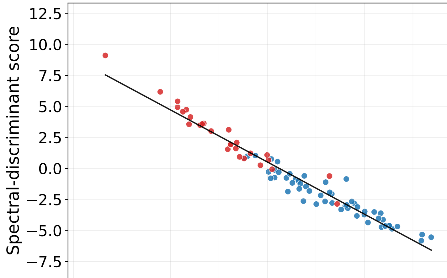
PZ — NUTS (posterior mean) r = -0.977 [-0.985, -0.964] , n = 81
