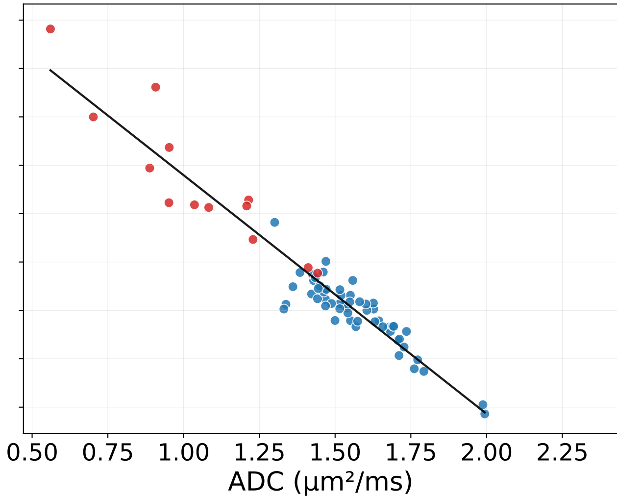
TZ — MAP ( \lambda = 10^{-3} ) r = -0.959 [-0.976, -0.930] , n = 68
