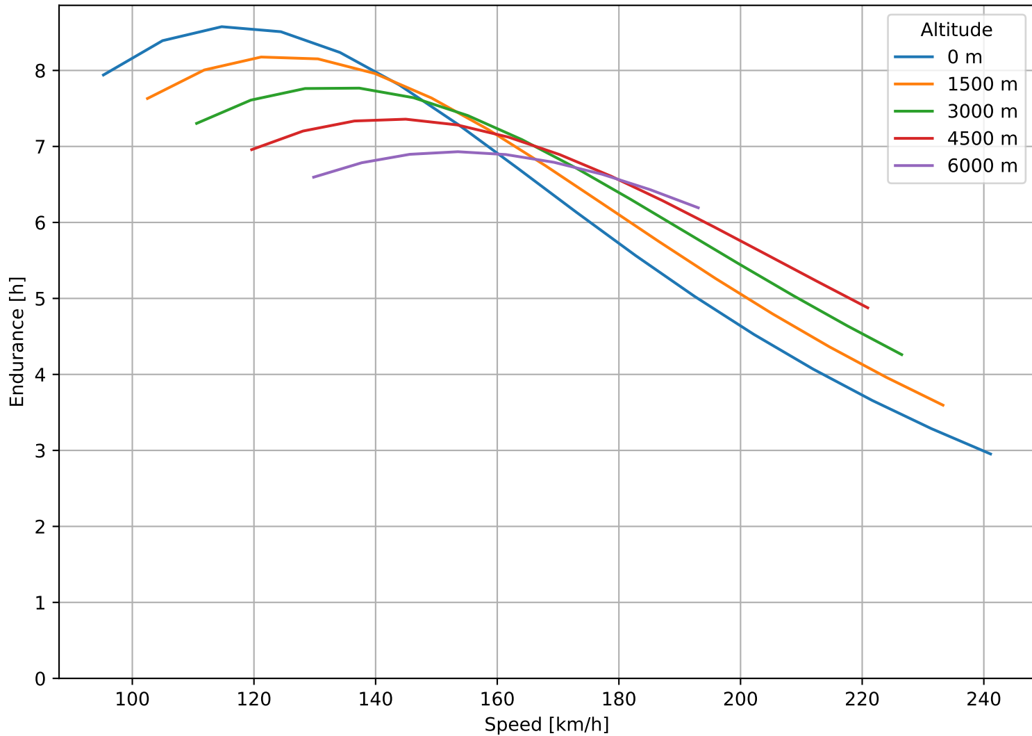
Endurance vs Speed: C-172
