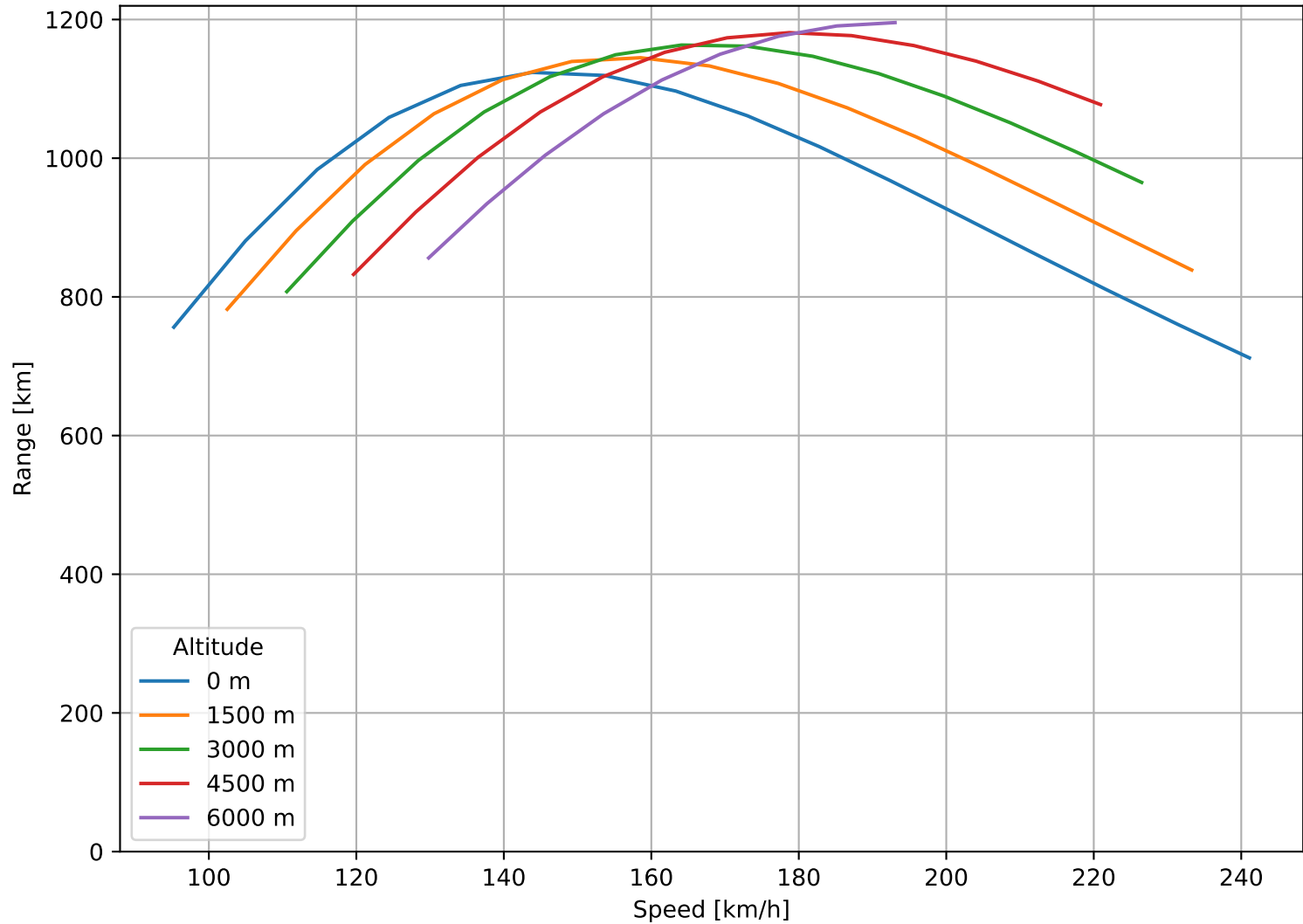
Range vs Speed: C-172
