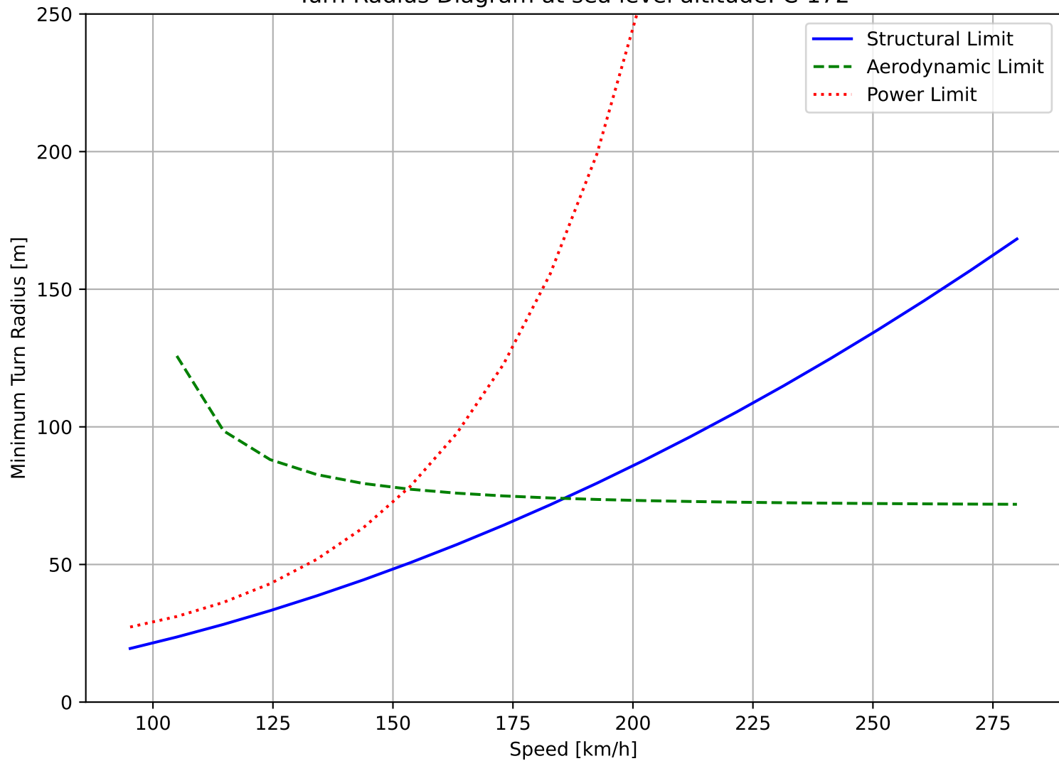
Turn Radius Diagram at sea level altitude: C-172
