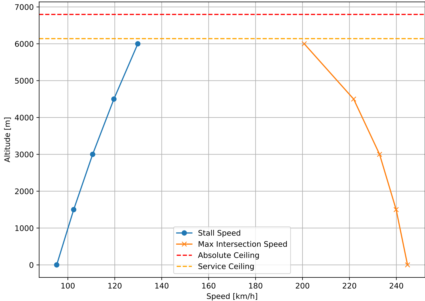
Flight Envelope: C-172
