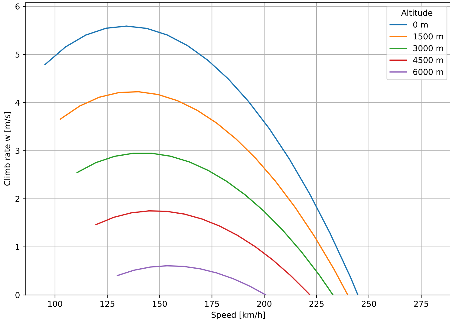
Climb Rate vs Speed: C-172
