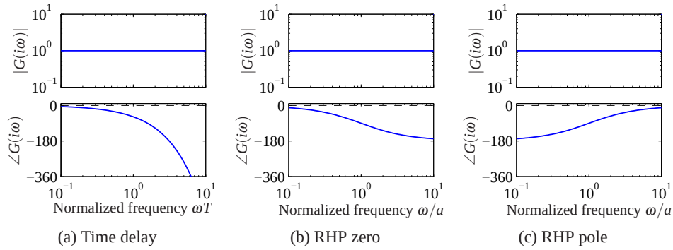
Figure 9.13: Bode plots of systems that are not minimum phase. (a) Time delay G(s) = e^{-sT} , (b) system with a right half-plane (RHP) zero G(s) = (a-s)/(a+s) and (c) system with right half-plane pole. The corresponding minimum phase system has the transfer function G(s) = 1 in all cases, the phase curves for that system are shown as dashed lines.
