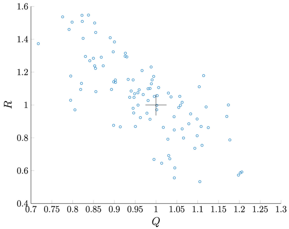
FIGURE 5. Q and R estimation for Case 2.
