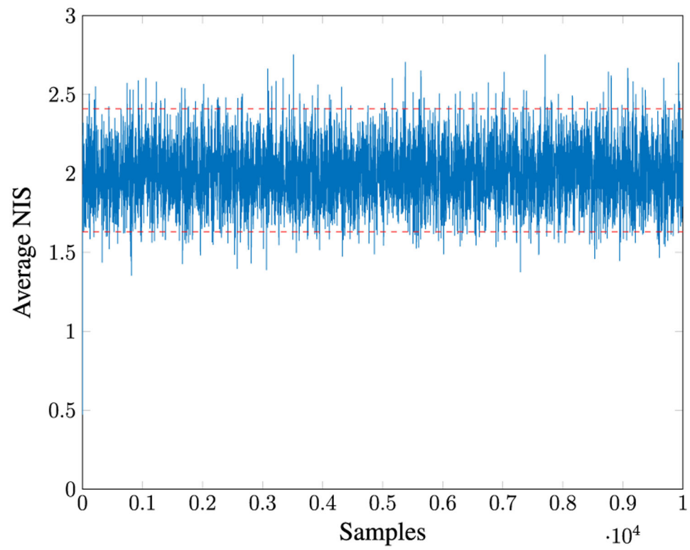
FIGURE 9. Averaged NIS for Case 3.
