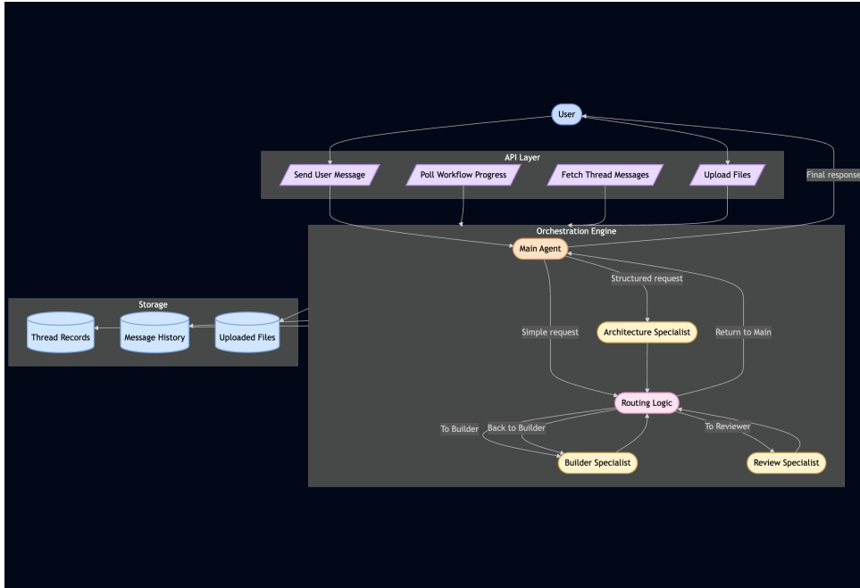
Figure 3: Application architecture
