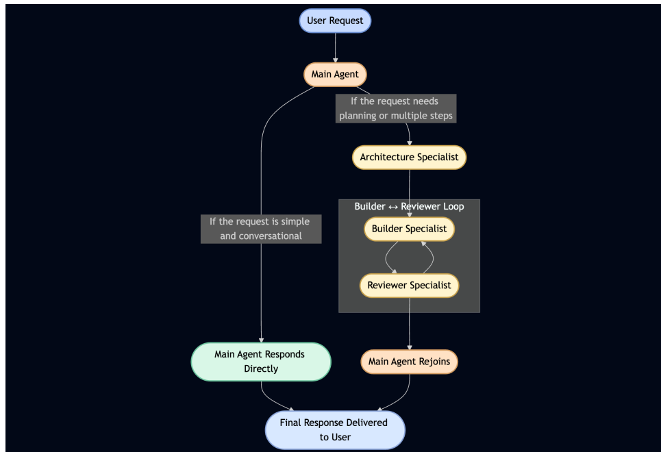
Figure 2: Workflow diagram
