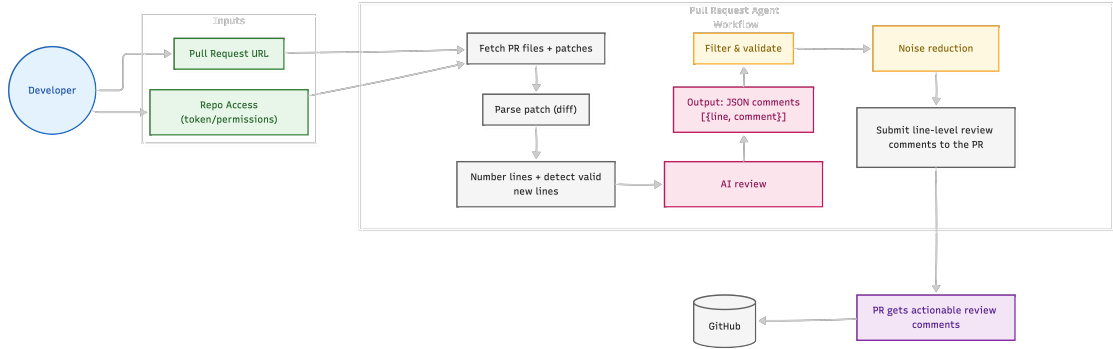
Figure 4: Pull request agent's workflow
