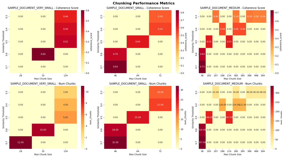
Figure 3: Threshold and maximum chunking tests
