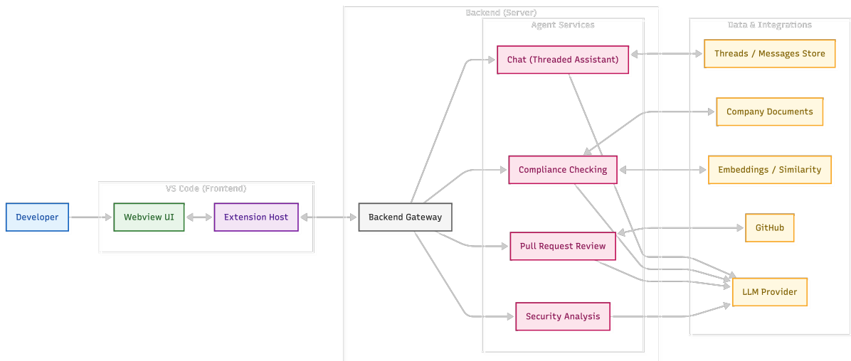
Figure 7: Application architecture
