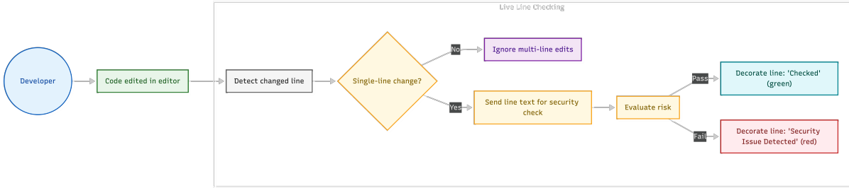
Figure 5: Workflow diagram for Security Agent
