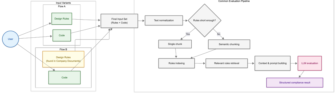
Figure 2: Rules Check agent’s workflow
