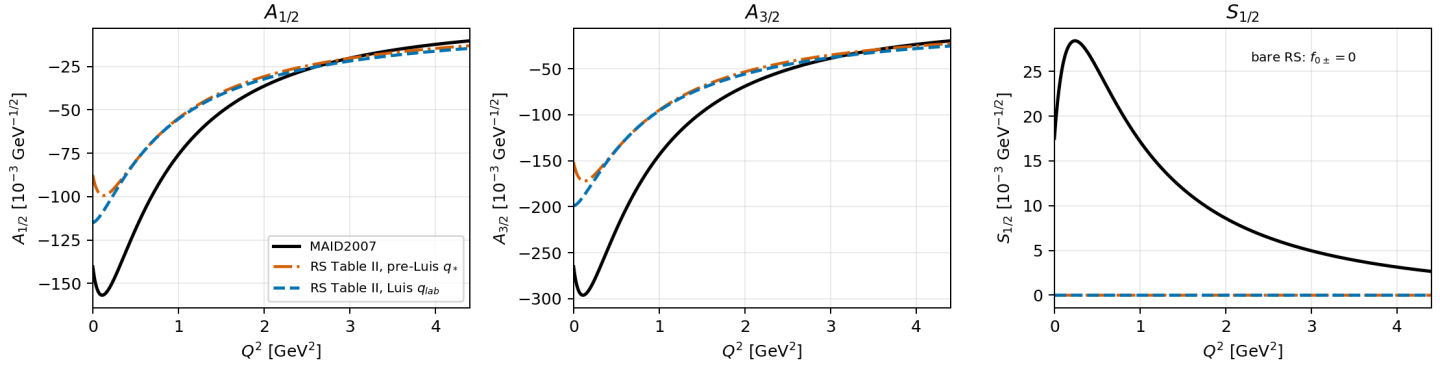
Original Rein-Sehgal P33 f amplitudes converted to A/S
