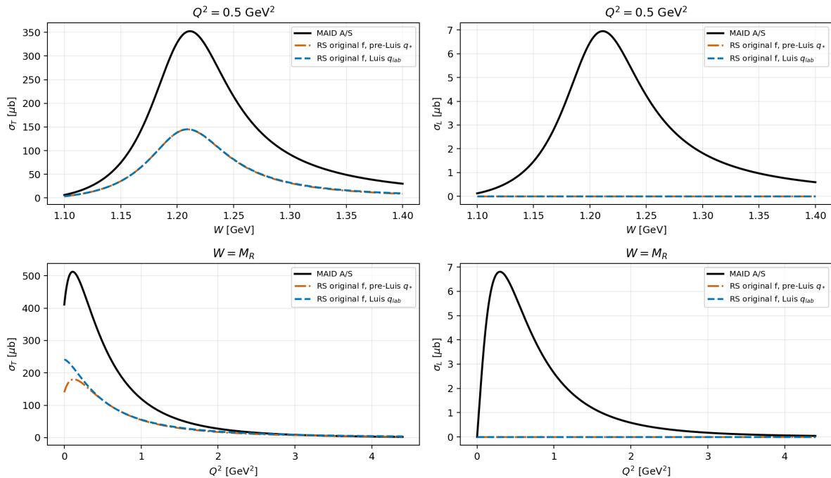
Original Rein-Sehgal P33 f-amplitude cross sections vs MAID
