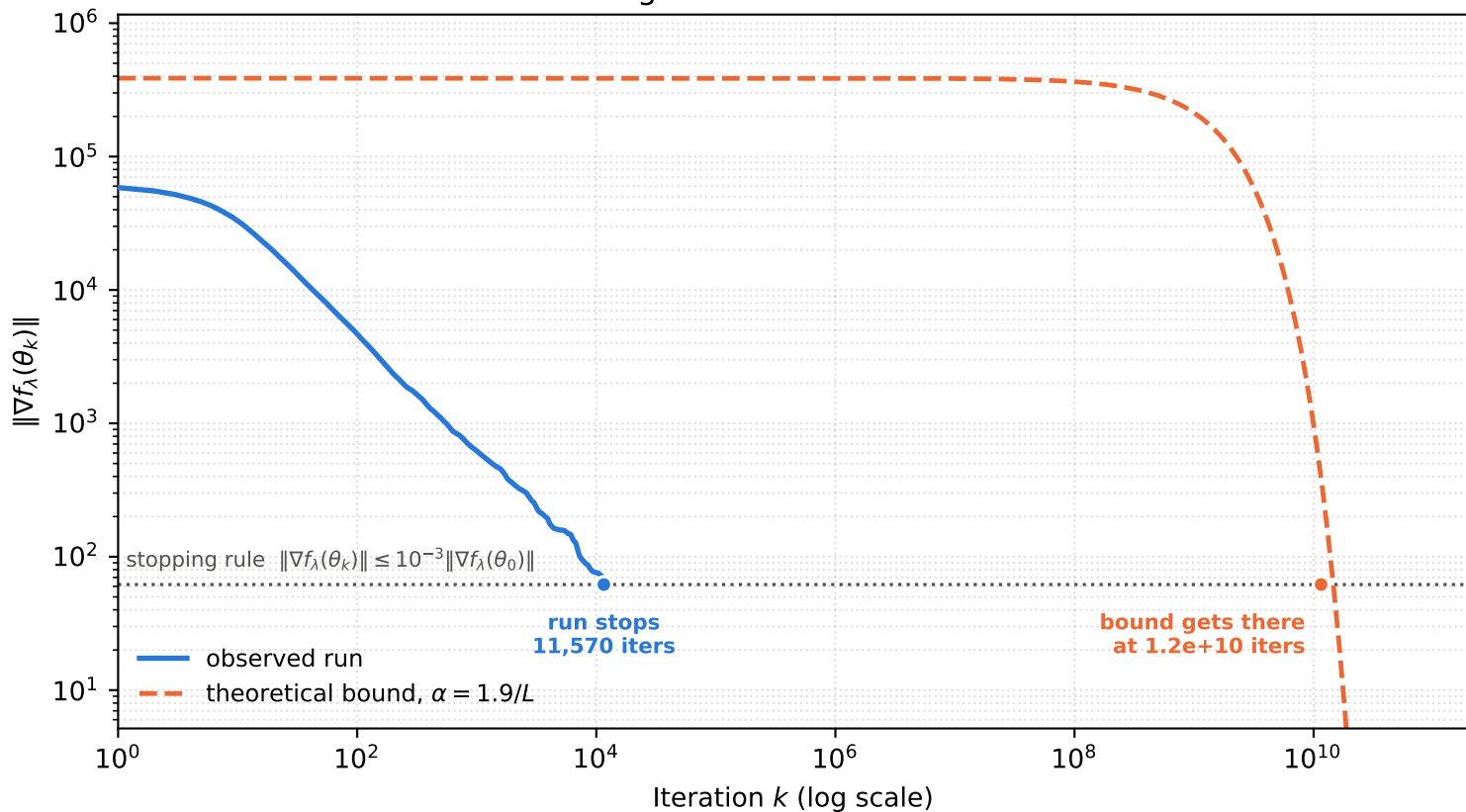
Convergence over the full horizon
