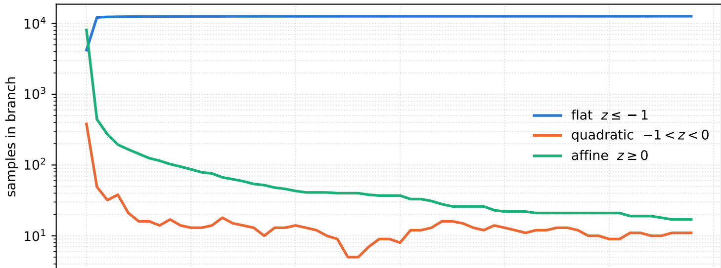
Which branch of \phi the margins occupy
