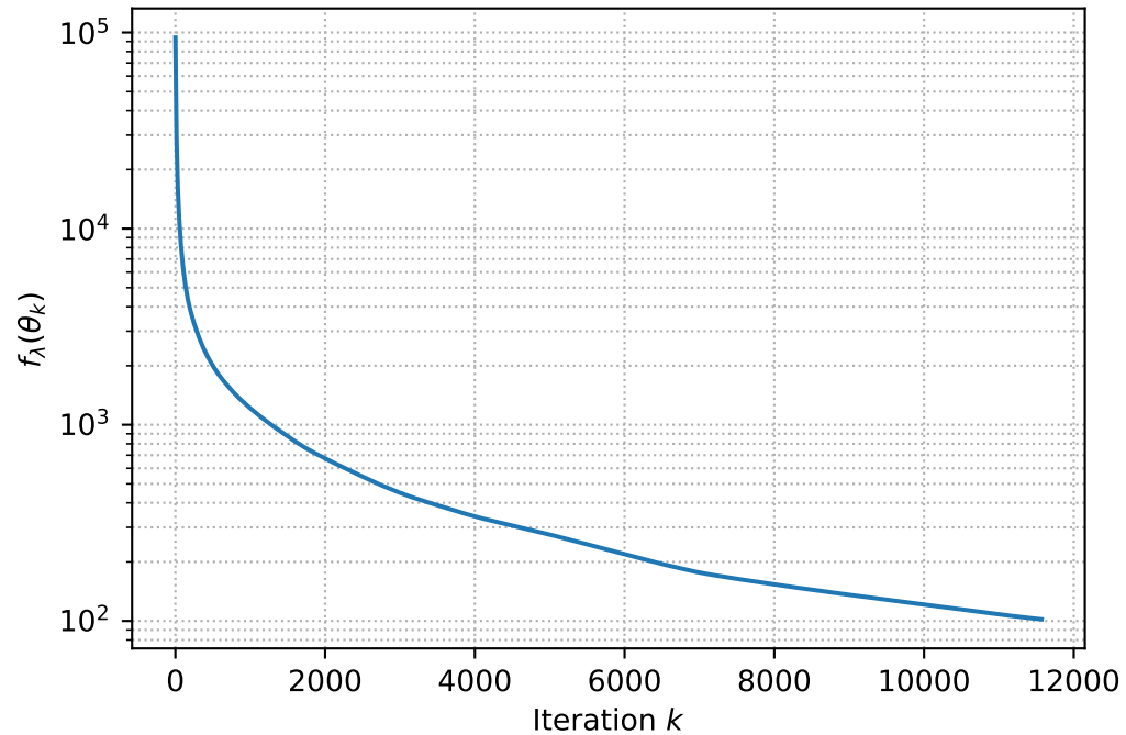
Objective value
