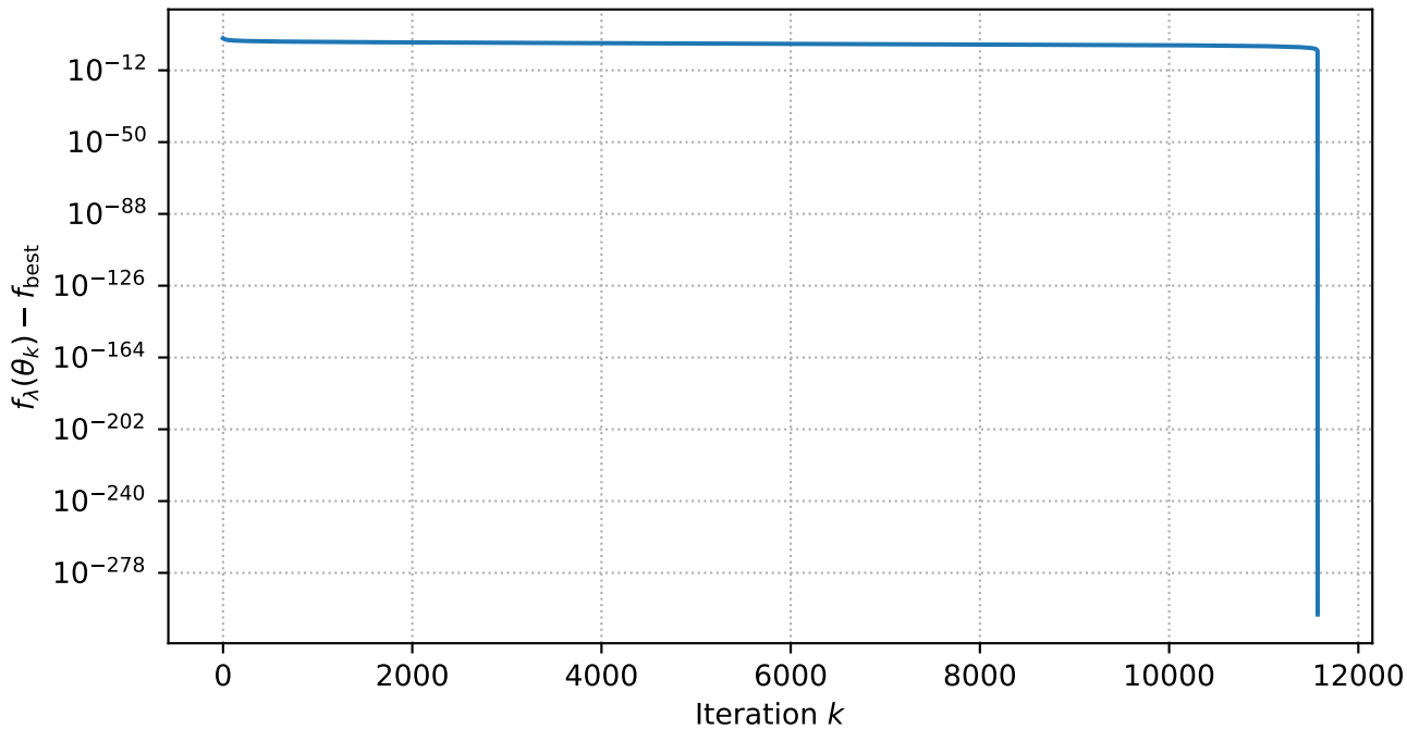
Objective gap to best observed value
