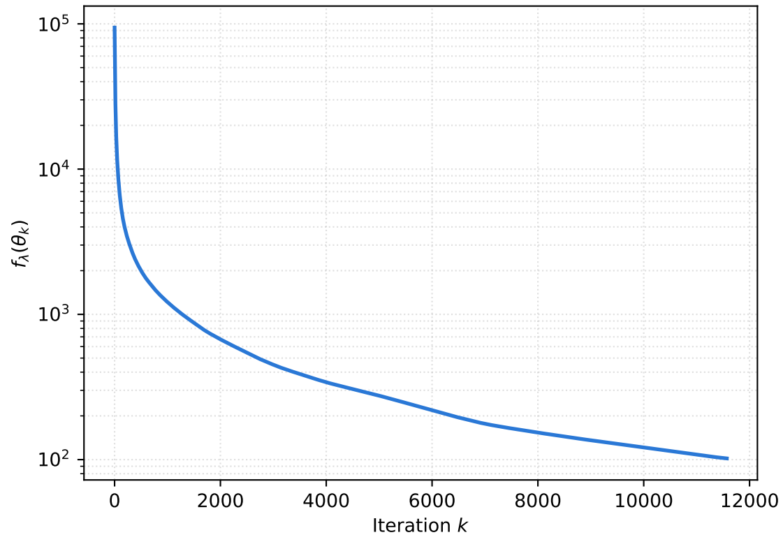
Objective value
