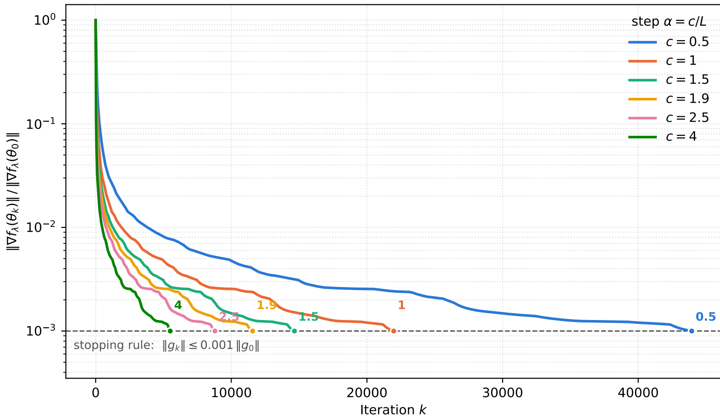
Gradient-norm decay for \alpha = c/L (seed 42)
