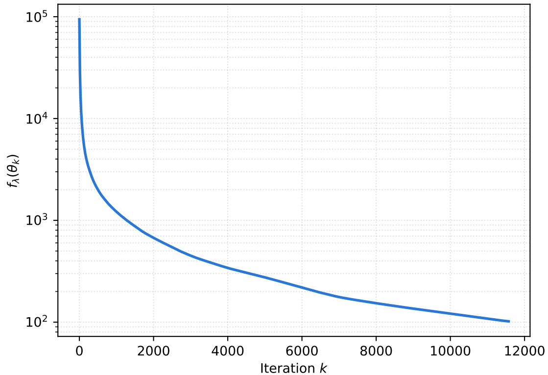
Objective function
