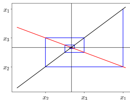
(b) Cobweb diagram for the function f(x) = ax when a = -0.5
