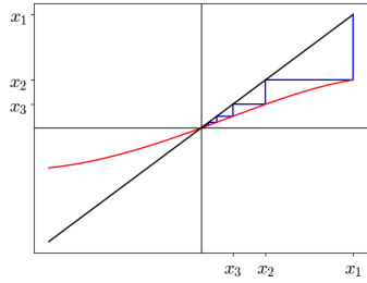
(a) \lambda < 0
