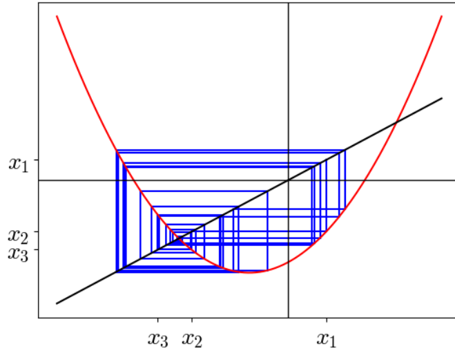
Figure 1.6: Cobweb diagram for the function f(x) = x^2 - 2 + x
