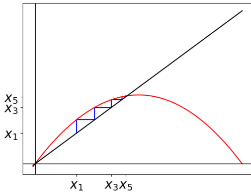
(a) Cobweb diagram for the function f(x) = 1.8x(1 - x) taking x_0 < 0.5
