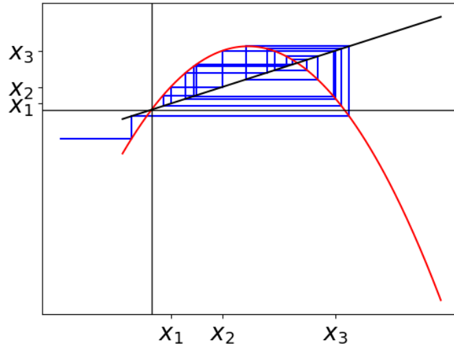
Figure 3.9: We can observe the presence of chaos in the orbit of the logistic equation when \lambda > 4
