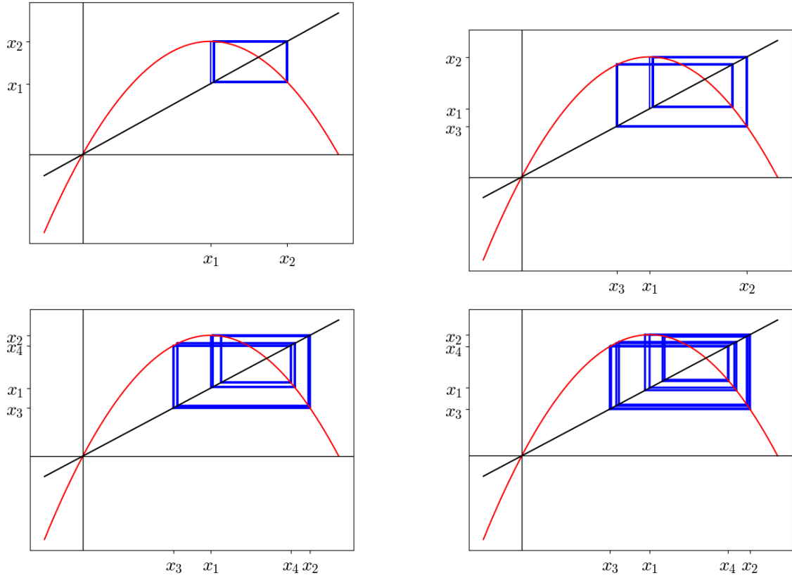
Figure 3.6: Representation of asymptotically stable periodic orbits of periods 2, 4, 8, 16 where the logistic equation takes values \lambda = 3.2 , \lambda = 3.52 , \lambda = 3.55 , \lambda = 3.567 ; the first 100 iterations have been removed
