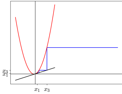
(c) Cobweb diagram for the function f(x) = x + x^2 starting from x_0 = 1
