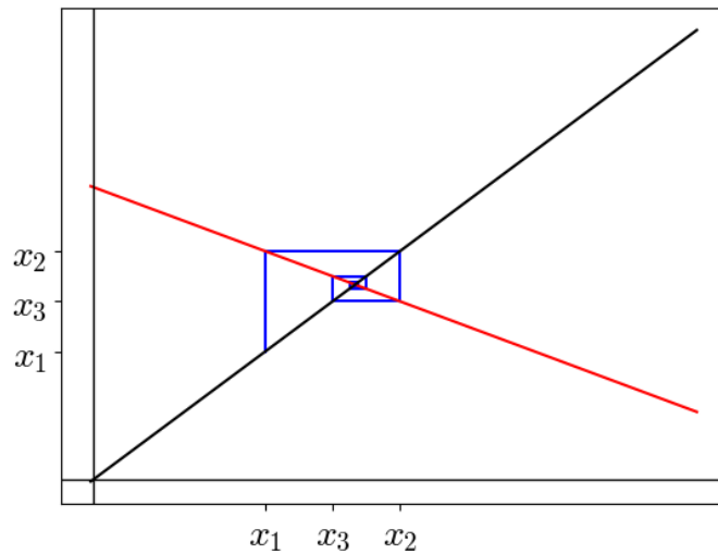
Figure 1.4: Cobweb diagram for the function f(x) = x + bx(1 - x) with b = 1.3 and x_0 = 0.567
