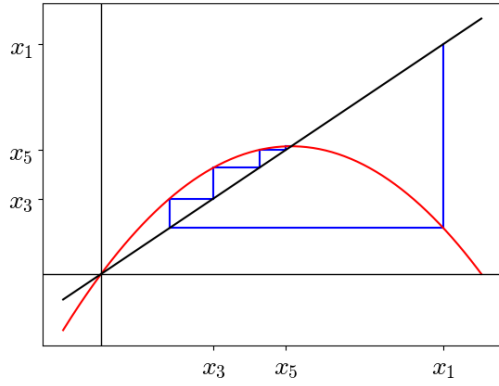
(a) Cobweb diagram of the logistic equation when a = 2
