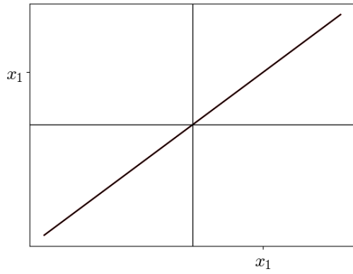
(a) Cobweb diagram for the function f(x) = ax when a = 1
