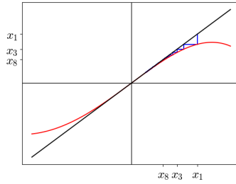
(b) \lambda = 0
