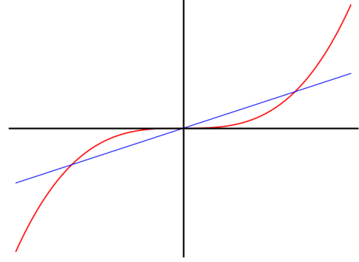
(b) Representation of G_\lambda(x) in the particular case G_\lambda(x) = x^3 together with the function f(x) = x ; the intersection points of f with G_\lambda(x) represent the fixed points of G_\lambda(x)
