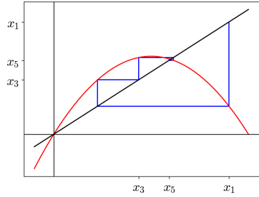
(b) Cobweb diagram of the logistic equation when a = 2.5
