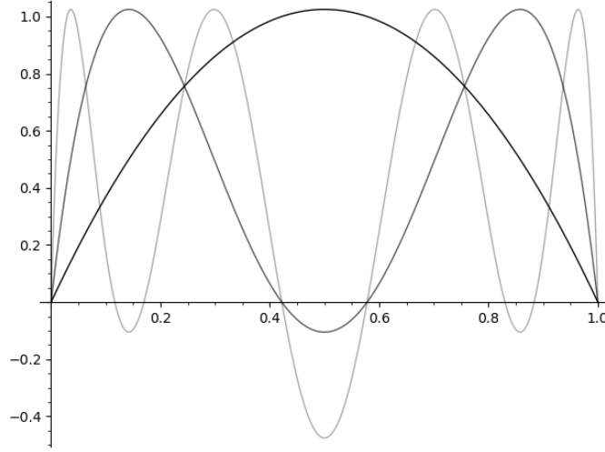
Figure 3.10: Graphical representation of f_\lambda(x) , f_\lambda^2(x) and f_\lambda^3(x)
