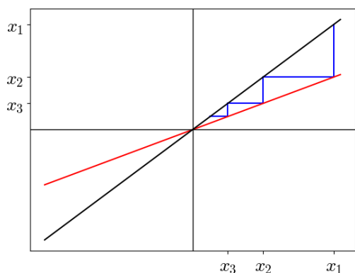
(a) Cobweb diagram for the function f(x) = ax when a = 0.5
