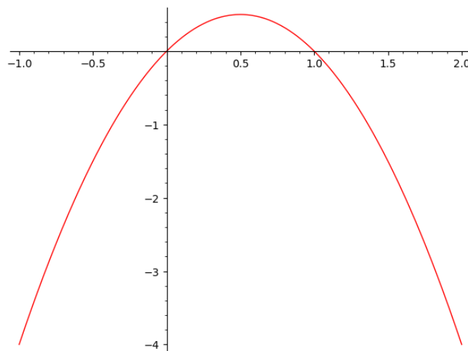
Figure 1.3: Logistic equation when a = 2 .
