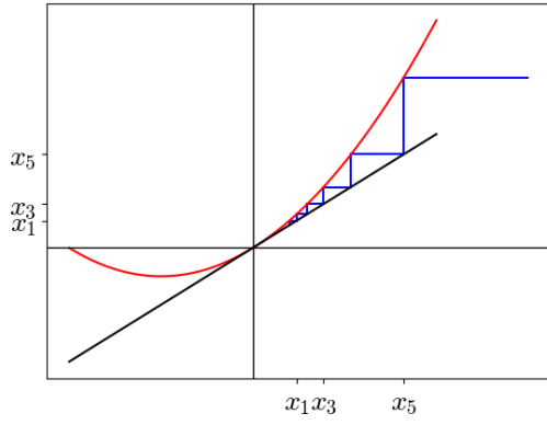
(a) Cobweb diagram for the function f(x) = x + x^2 starting from x_0 = 0.2
