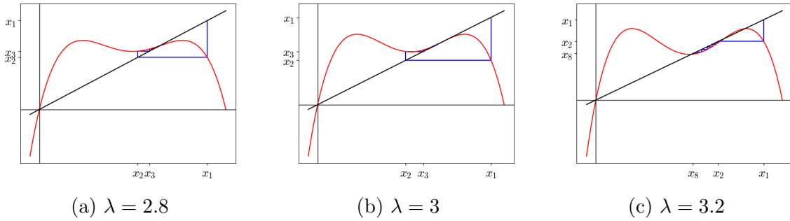
Figure 3.5: Study of fixed points of the second iteration of the logistic equation for \lambda = 2.8 , \lambda = 3 , \lambda = 3.2
