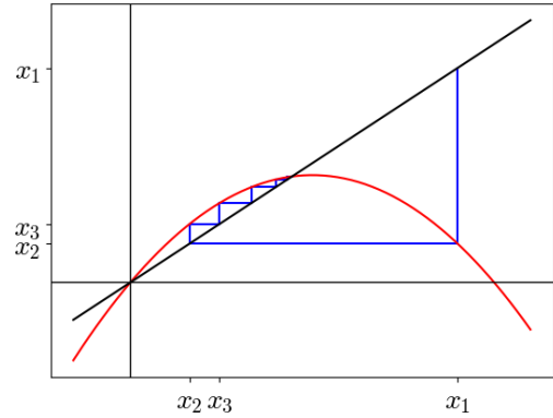
(b) Cobweb diagram for the function f(x) = 1.8x(1 - x) taking x_0 > 0.5
