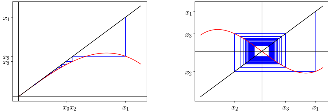
Figure 1.10: Cobweb diagrams for the functions f(x) = -x + x^3 and f(x) = x - x^3 starting from x_0 = 0.7
