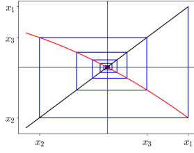
(a) Cobweb diagram for F(\lambda, x) = -(1 + \lambda)x - (3 + \lambda)x^2 with \lambda < 0
