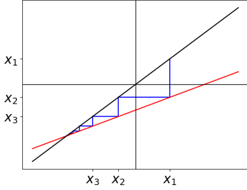
(a) Cobweb diagram for the function F(\lambda, x) = \lambda + 0.5x when \lambda < 0
