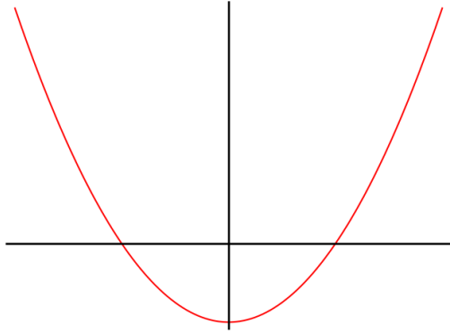
(a) Representation of T_\lambda(x) in the particular case T_\lambda(x) = x^2 - 1
