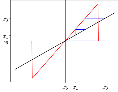
Figure 1.7: Cobweb diagram for the function f(x) = 2x when -5 < x < 5 and 0 otherwise, taking x_0 = 0.1 .
