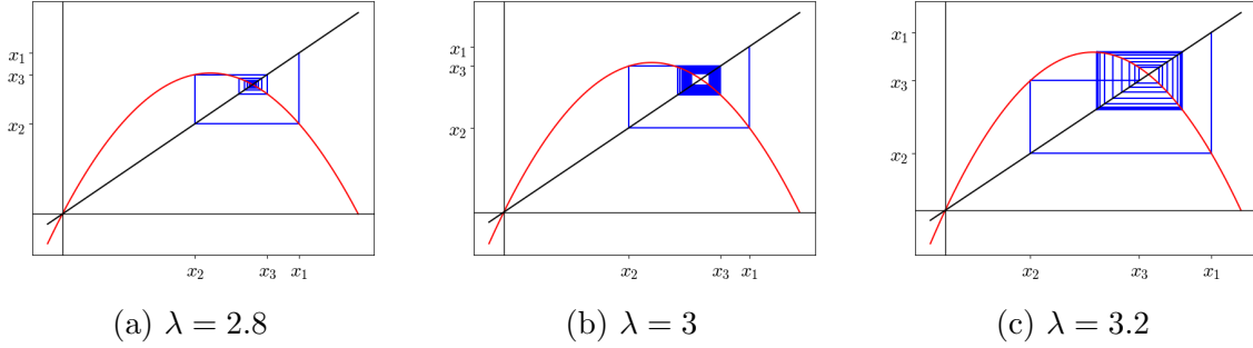
Figure 3.4: Study of fixed points of the logistic equation for \lambda = 2.8 , \lambda = 3 , \lambda = 3.2
