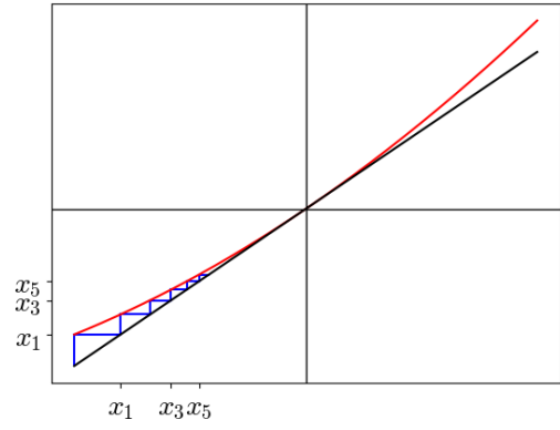
(b) Cobweb diagram for the function f(x) = x + x^2 starting from x_0 = -0.2
