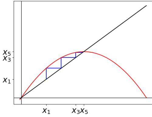
(a) Cobweb diagram for the function f(x) = 2x(1-x) taking x_0 < 0.5
