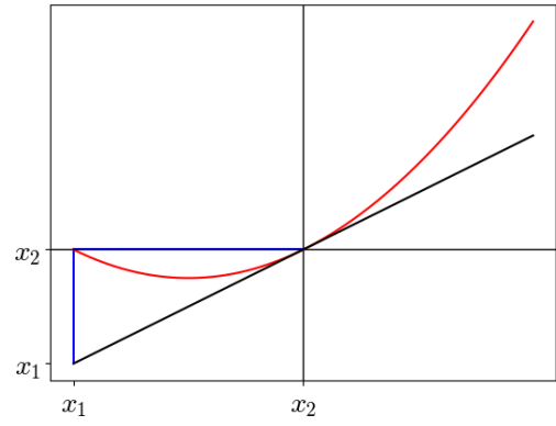
(d) Cobweb diagram for the function f(x) = x + x^2 starting from x_0 = -1
