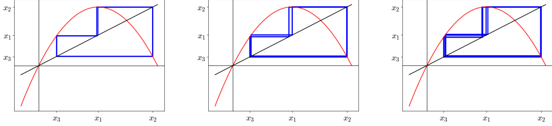
Figure 3.8: Representation of asymptotically stable periodic orbits of periods 3, 6, 12, where the logistic equation takes values \lambda = 3.839 , \lambda = 3.845 , \lambda = 3.849 . The first 100 iterations have been removed.
