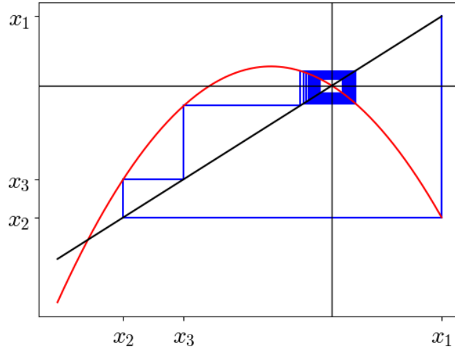
Figure 1.9: Cobweb diagram for f(x) = -x - 3x^2 taking as initial value x_0 = 0.3
