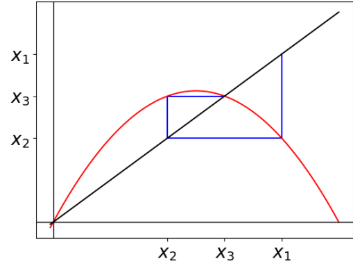
(b) Cobweb diagram for the function f(x) = 2.5x(1-x) taking x_0 > 0.5
