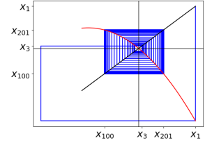
(c) Cobweb diagram for F(\lambda, x) = -(1 + \lambda)x - (3 + \lambda)x^2 with \lambda > 0
