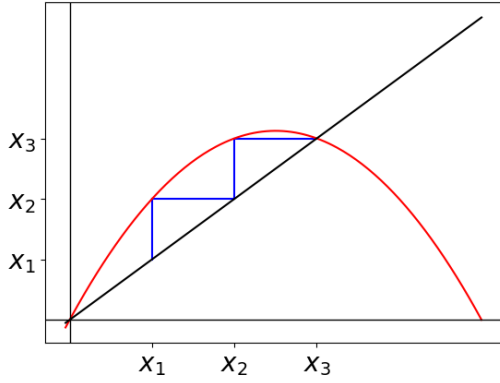
(a) Cobweb diagram for the function f(x) = 2.5x(1-x) taking x_0 < 0.5
