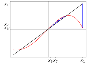
(c) \lambda > 0
