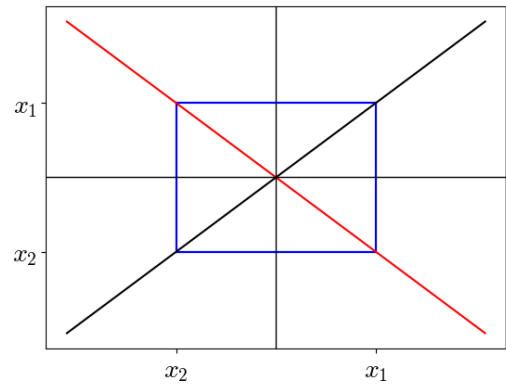
(b) Cobweb diagram for the function f(x) = ax when a = -1
