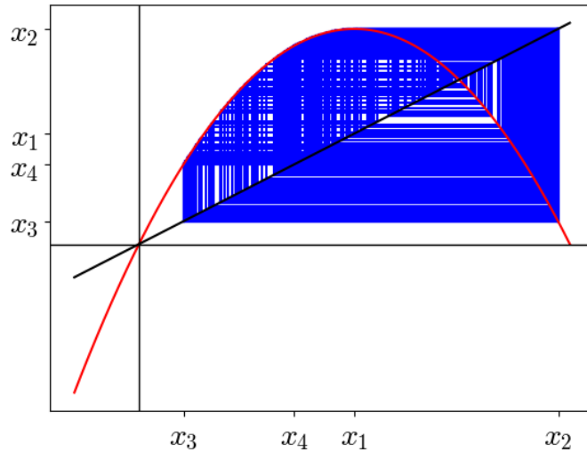
Figure 3.7: We can observe the presence of chaos in the orbit of the logistic equation when \lambda = 3.891
