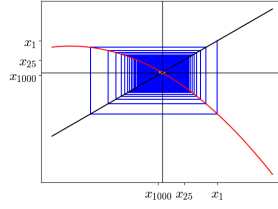
(b) Cobweb diagram for F(\lambda, x) = -(1 + \lambda)x - (3 + \lambda)x^2 with \lambda = 0
