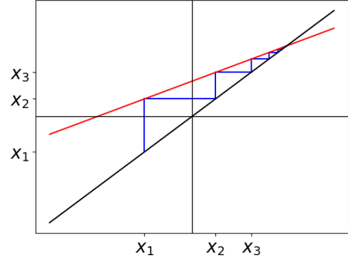
(b) Cobweb diagram for the function F(\lambda, x) = \lambda + 0.5x when \lambda > 0
