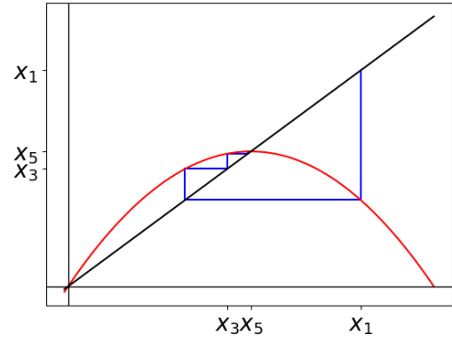
(b) Cobweb diagram for the function f(x) = 2x(1-x) taking x_0 > 0.5
