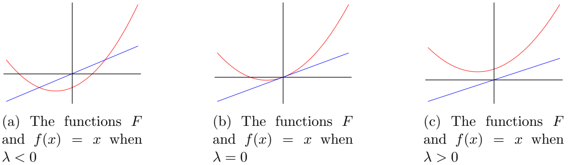
Figure 2.3: General representation of the functions F and f(x) = x for different values of \lambda .
