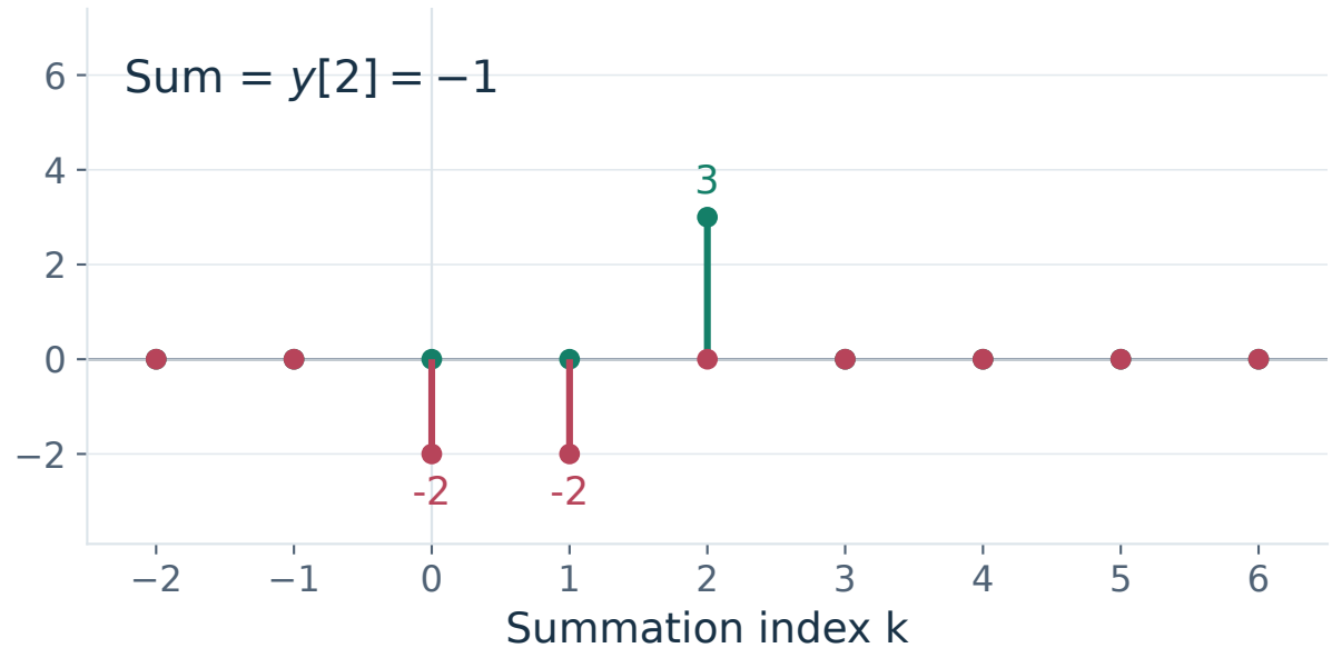
Products x[k]h[n-k]
