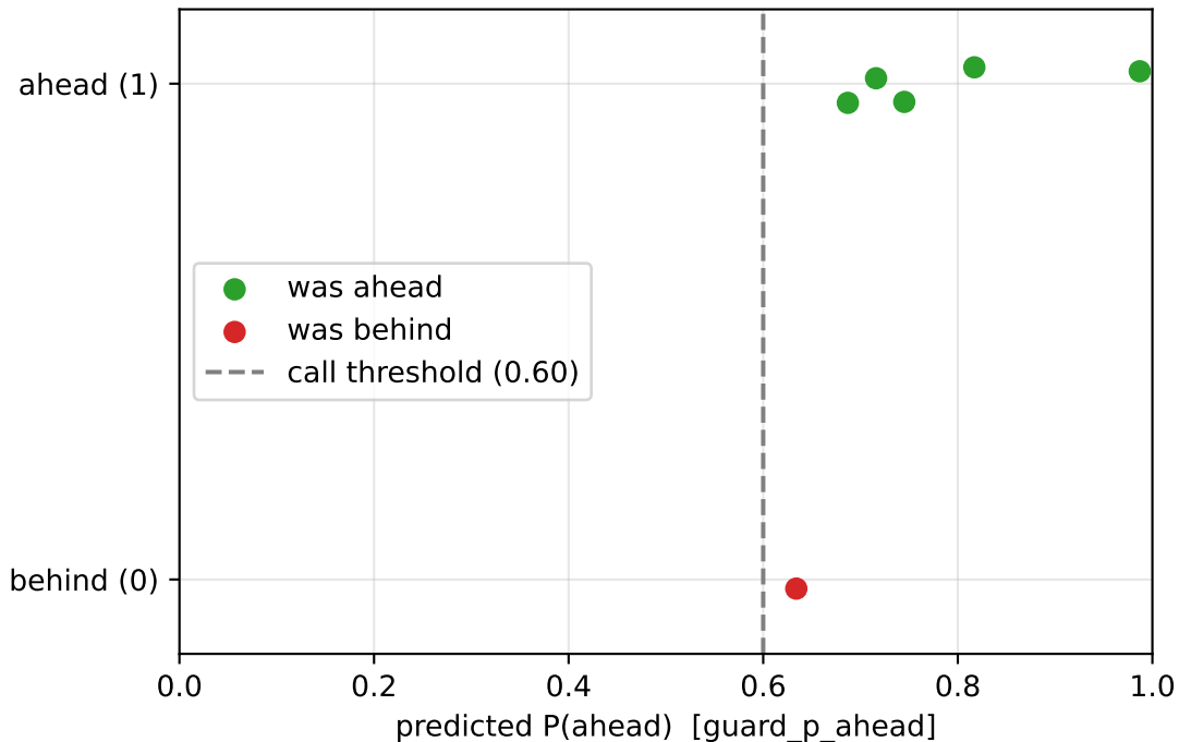
Per-call guard calibration — 6 Bayesian calls
