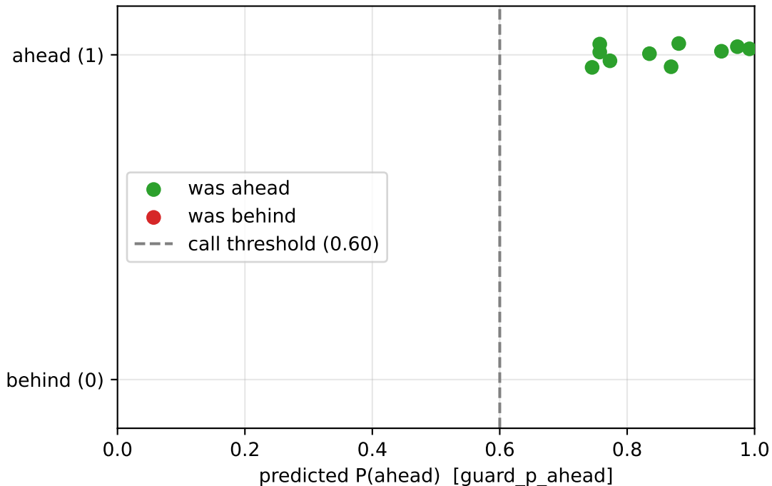
Per-call guard calibration — 10 Bayesian calls
