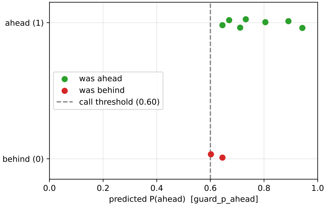
Per-call guard calibration — 9 Bayesian calls
