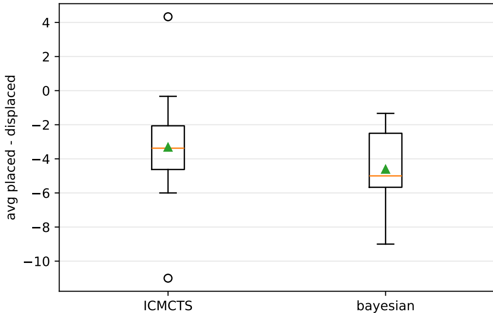
Swap quality (value delta, negative = improvement)
