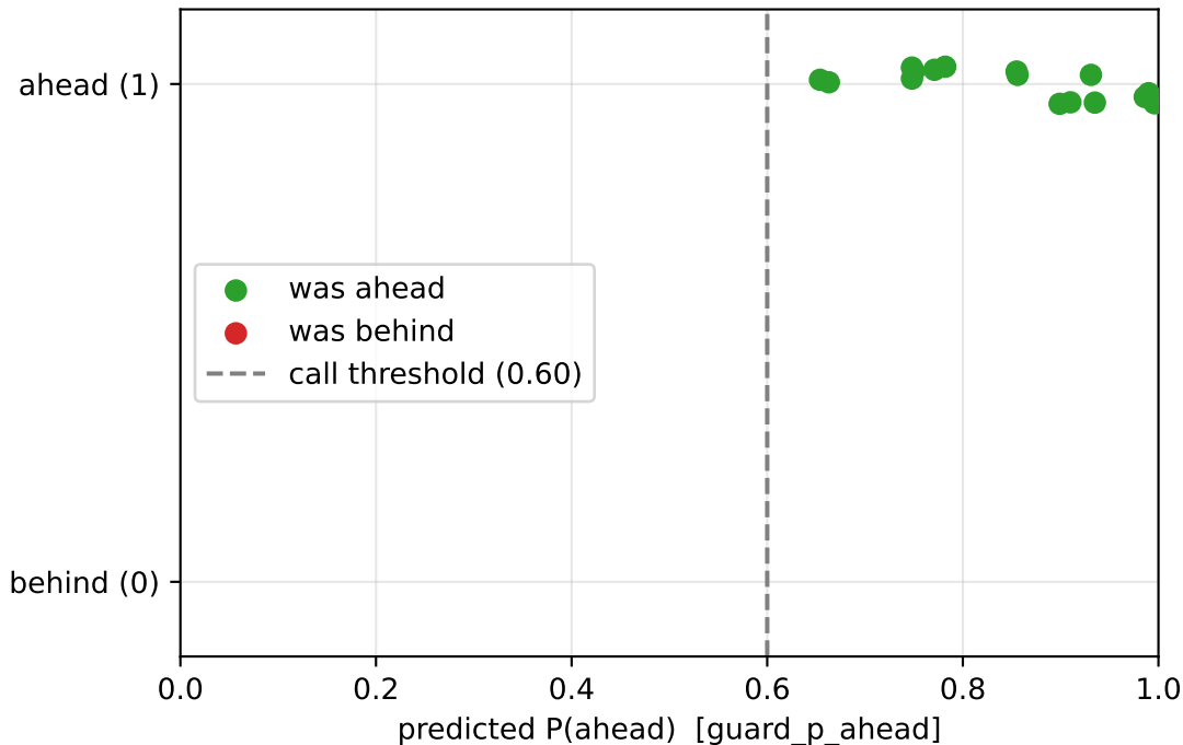
Per-call guard calibration — 16 Bayesian calls
