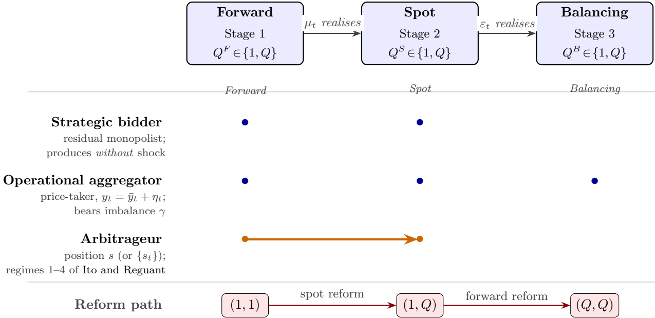
Figure 1: Sequential markets, granularity, and agents. Forward \rightarrow Spot \rightarrow Balancing, each with its own granularity Q^m \in \{1, Q\} ; information resolves between stages. Blue dots: which agents act at which stages. Orange: arbitrageur position s linking forward to spot. Bottom: the auction-side reform path (1, 1) \rightarrow (1, Q) \rightarrow (Q, Q) .
