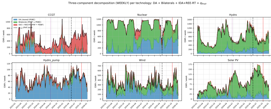
Figure 6: Weekly three-component decomposition per technology, Big-4 aggregate. PDBC (blue) + Bilaterals (green) + IDA + REE-RT (red) = q_{\text{final}} (PHF, black). CCGT’s blue layer collapses post-blackout while red balloons. Vertical guides: MTU15-IDA, Blackout, MTU15-DA.
