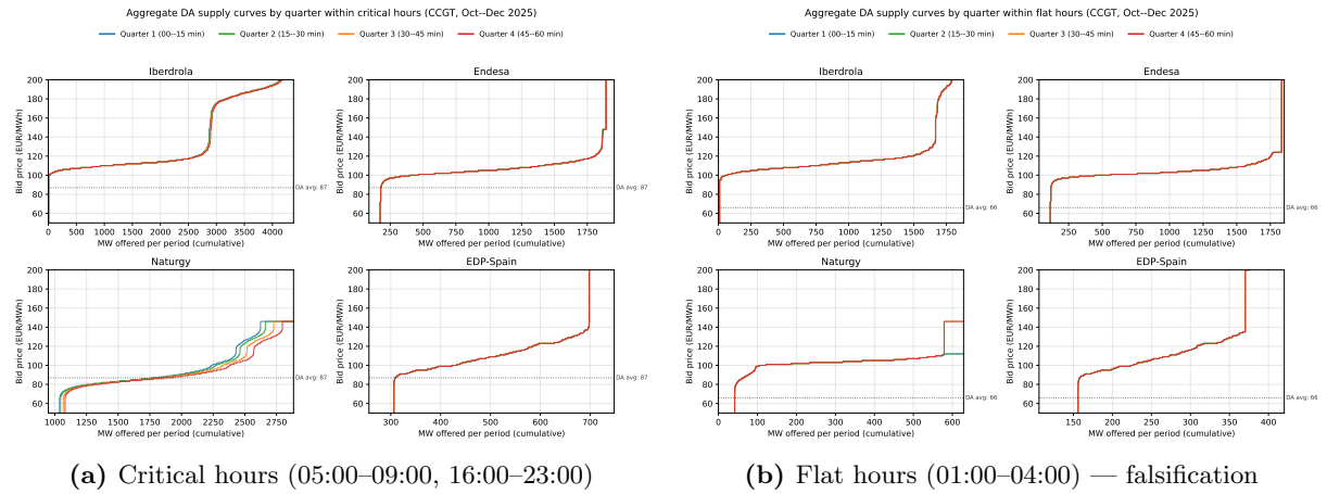
Figure 3: Aggregate DA supply curves by within-hour quarter, CCGT per firm, Oct–Dec 2025.
