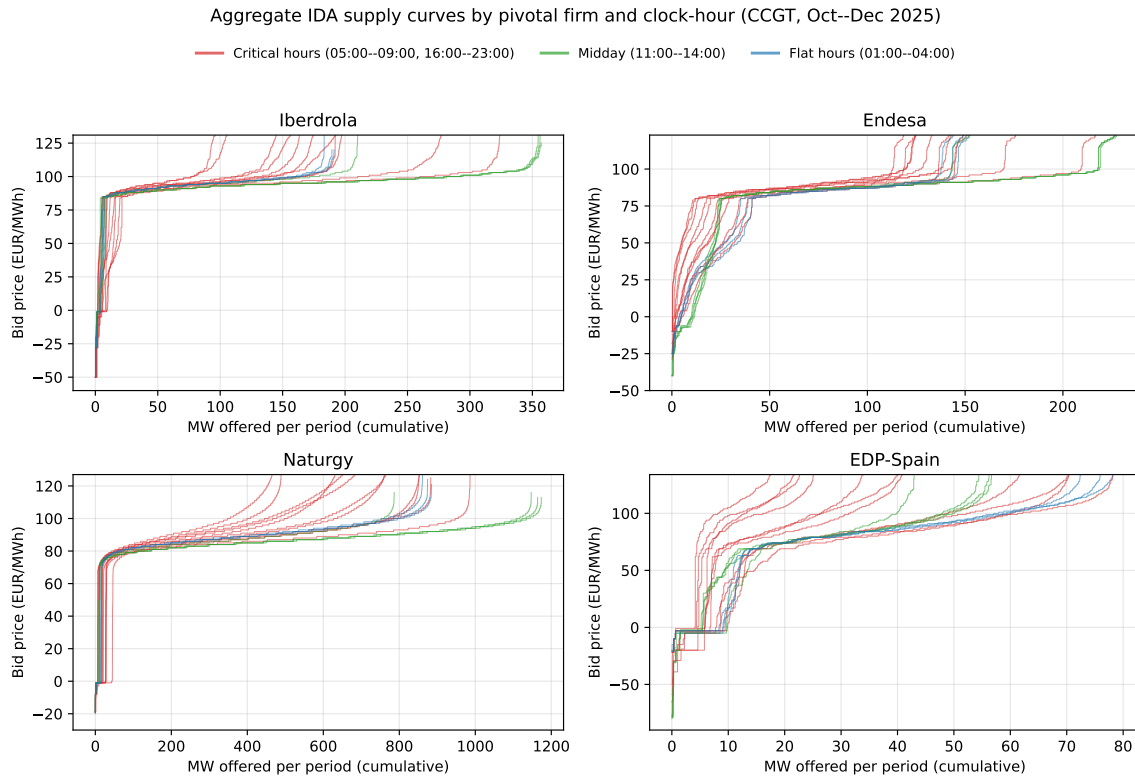
Figure 9: Aggregate IDA supply curves by pivotal firm and clock-hour, CCGT, October–December 2025. Same construction as Figure 4 on ICAB+IDET data, pooled across the 3 IDA sessions.
