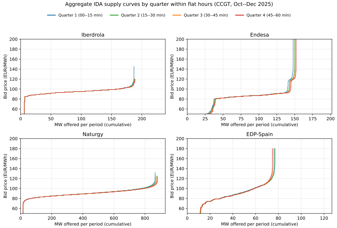
Figure 11: Aggregate IDA supply curves by quarter within flat hours, CCGT.
