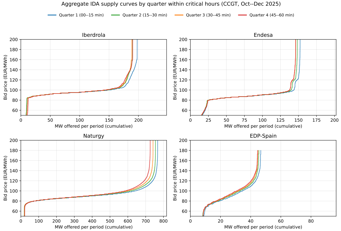
Figure 10: Aggregate IDA supply curves by quarter within critical hours, CCGT.
