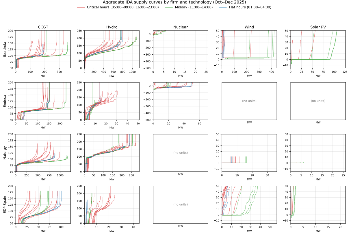
Figure 12: Aggregate IDA supply curves by firm and technology, by hour-class. Compact grid; same construction as Figure 14 on IDA data.
