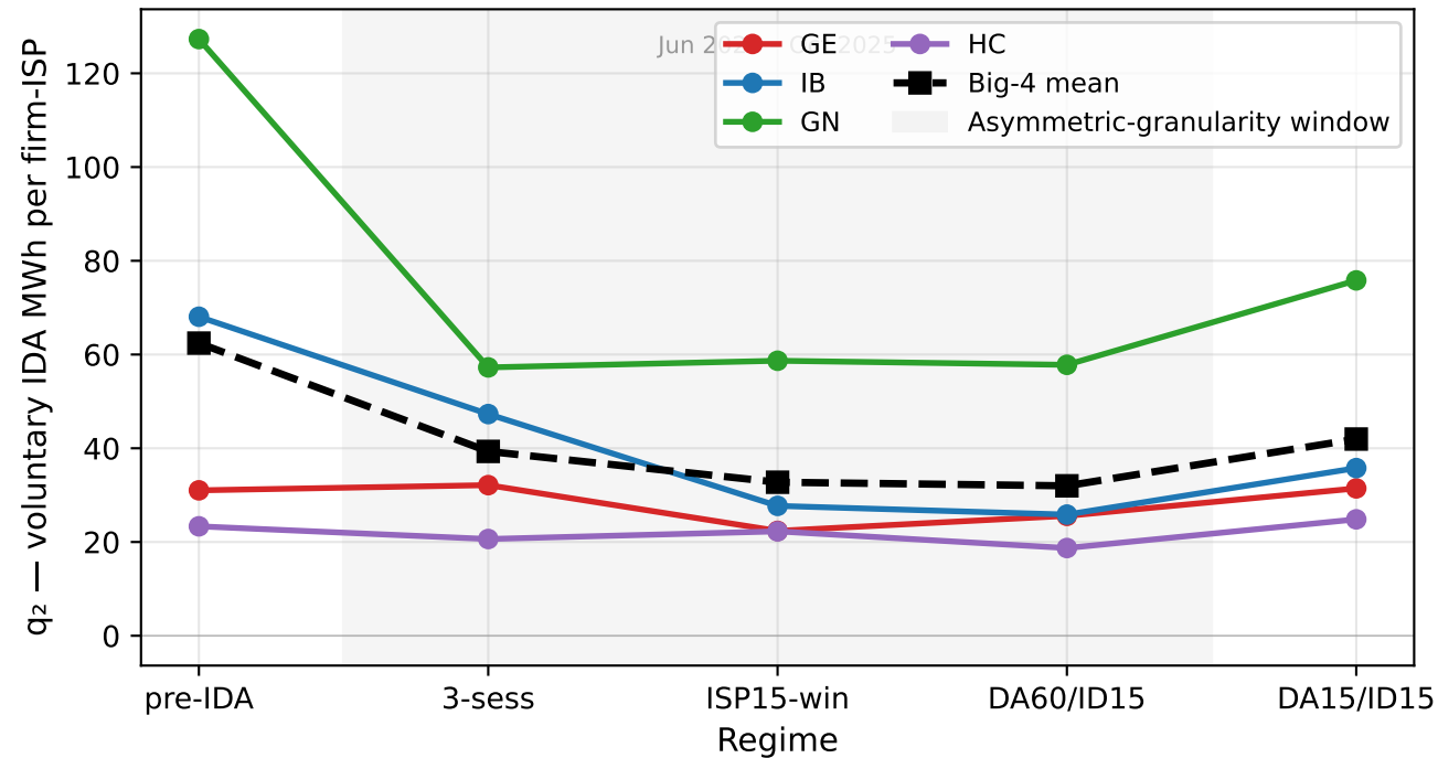
Big-4 q 2 trajectory at firm-ISP-replicated grain (IR-cleanest strategic-spot measure, max disaggregation)
