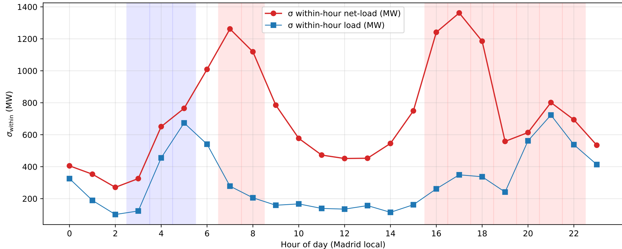
Within-hour standard deviation of (net-)load by hour, Spain 2025
