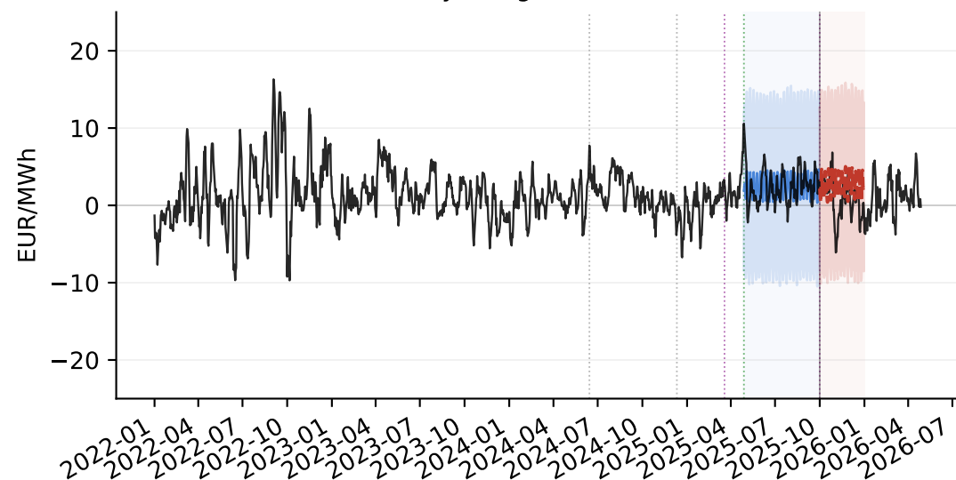
DA15 REAL: DA – IDA daily wedge, BSTS
