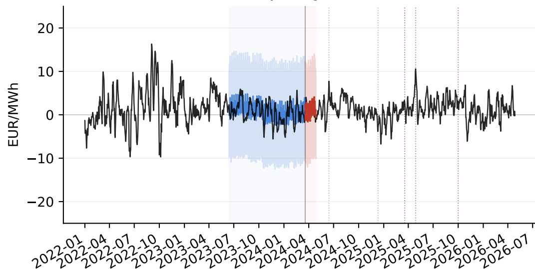
ID15 PLACEBO: DA – IDA daily wedge, BSTS
