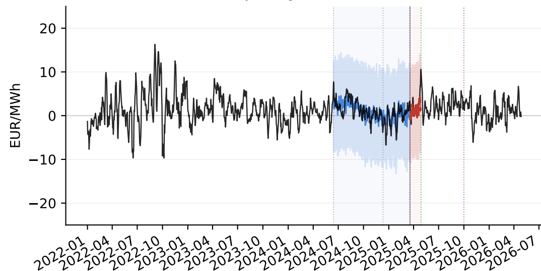
ID15 REAL: DA – IDA daily wedge, BSTS
