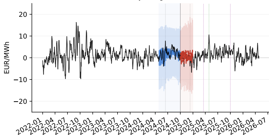
DA15 PLACEBO: DA – IDA daily wedge, BSTS
