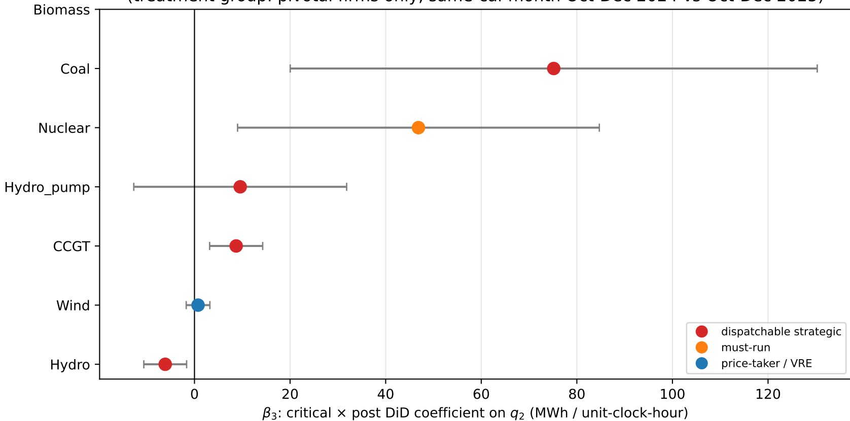
Treatment-effect heterogeneity by technology (treatment group: pivotal firms only, same-cal-month Oct-Dec 2024 vs Oct-Dec 2025)
