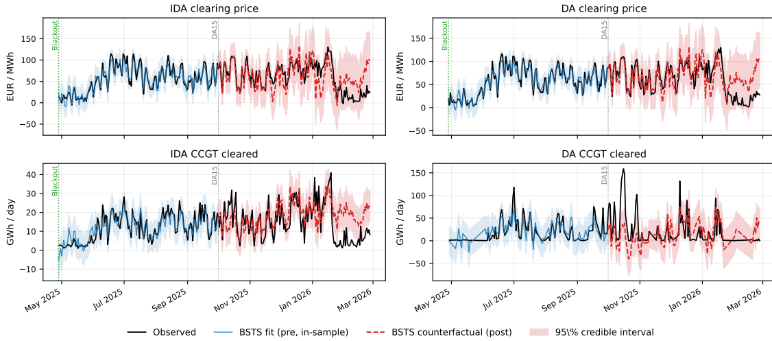
Figure 3: DA15 effects on both markets (2×2 zoomed view, post-window through 2026-02-26). Same colour scheme as Figure 2. Cutover 2025-10-01; reforzada-constant pre-window starts 2025-04-28. The DA CCGT panel (bottom-right) is the one quantity outcome where the observed series visibly departs from the counterfactual post-cutover — the surviving CCGT scale-up of finding (iii). By contrast, the IDA panels show no backwards transmission (intraday clearing follows day-ahead, so a DA-side reform cannot propagate backwards).
