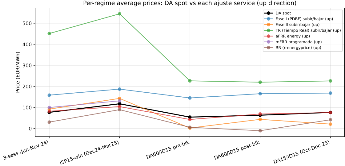
Figure 22: Prices vs DA across services. Lines: DA spot (black, reference) and each ajuste service. Y-axis: EUR/MWh.
